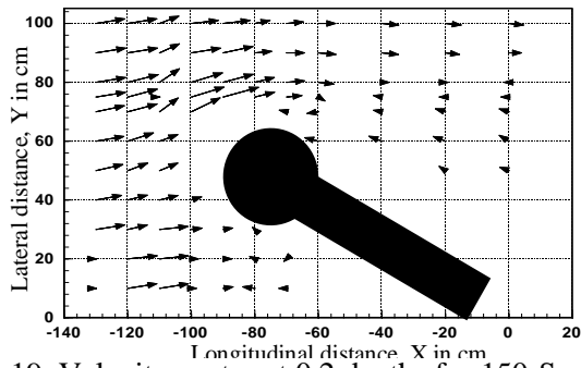
Fig.19. Velocity vector at 0.2 depths for 150-S-150
