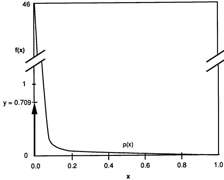
Figure 5: Failure Profile of the Circuit
