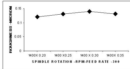
Fig.5. Feed rate Vs Roughness at 1400 RPM
