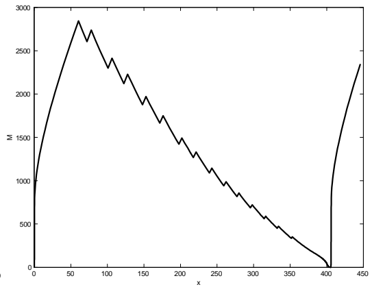
Fig.9-b \{M_n^{(2)}\}_{n \geq 0} for Problem 4
