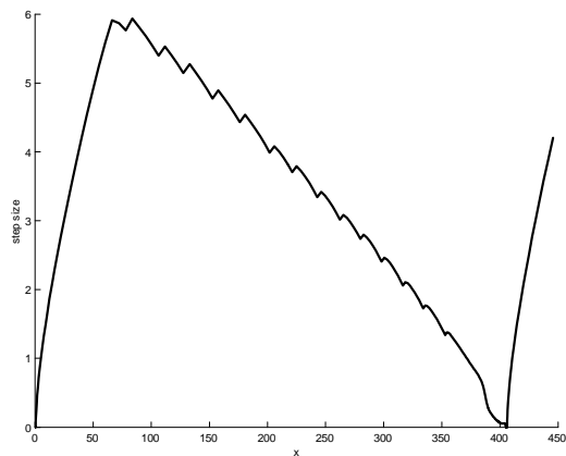
Fig.9-a Step size for Problem 4
