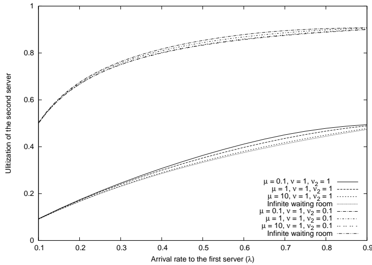
Fig. 2 Utilization of the second server vs. \lambda .
