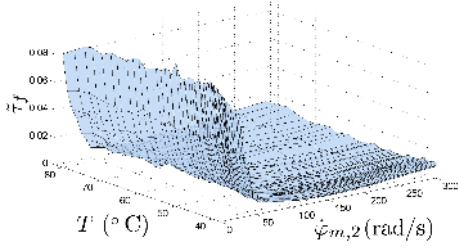
(a) Difference \bar{\tau}_f between the two static friction surfaces in Figure 7(a).
