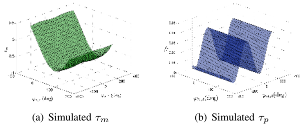
Fig. 4. Simulated joint load torques at joint 2. Notice the larger absolute values for \tau_m when compared \tau_p .
