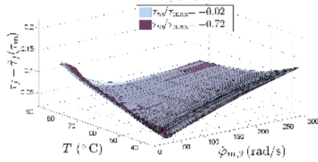
(b) Static friction surfaces in Figure 7(a) after subtraction of the \tau_m -dependent terms.
