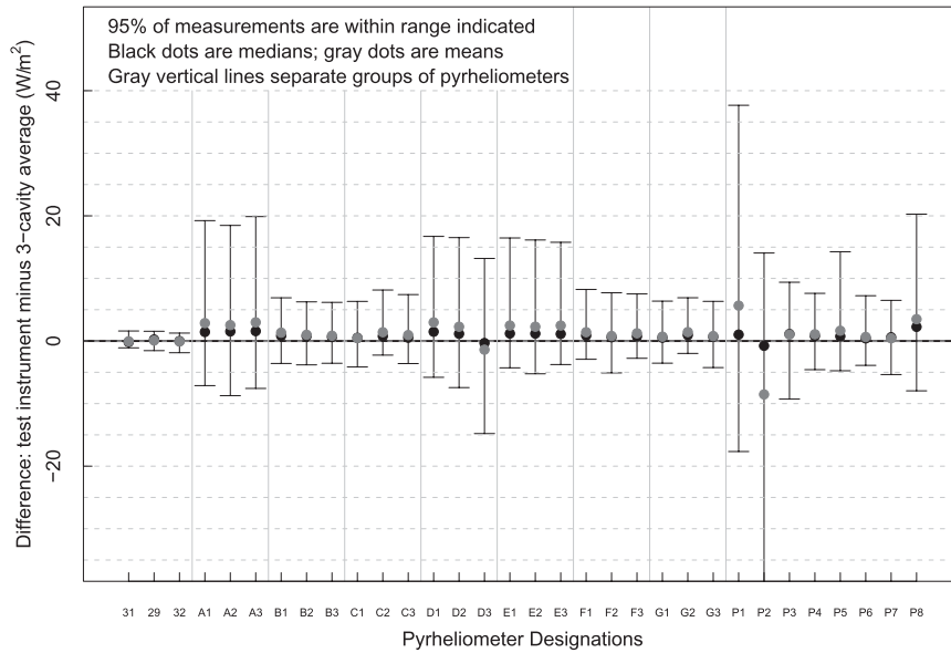
FIG. 5. Daytime data defined as points with the SZA < 91.2^\circ . The average direct irradiance is 410 \text{ W m}^{-2} . This plot reveals groups with similar behavior. Cavities perform the best and agree very well (see text for discussion of cavity results). Groups B, C, F, and G plus prototypes P4, P6, and P7 show similar and the best agreement with the cavities. Groups A, D, and E plus prototypes P3, P5, and P8 are similar and have the highest scatter and biases except for the outliers P1 and P2, which will not be discussed further.
