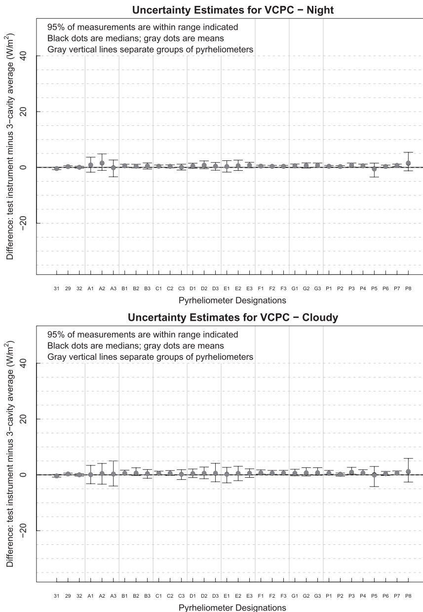
FIG. 4. (top) Nighttime results defined as all points with a SZA greater than 91.2^\circ . (bottom) Cloudy for SZAs <91.2^\circ and direct irradiance <4 \text{ W m}^{-2} (because a few instruments indicate nighttime data almost as high as this limit.) Some pyr heliometers show surprisingly high scatter even for 0 irradiance.
