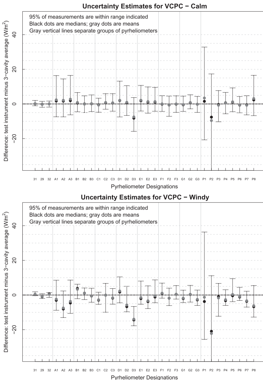
FIG. 8. Plots are for (top) calm and (bottom) windy conditions with direct irradiance > 700 \text{ W m}^{-2} . (top) Similar to Fig. 5. (bottom) Suggests that the wind produces negative offsets vis-à-vis calm circumstances; however, this is not always true and the instruments within groups showed independent behavior. The 95% ranges were similar within the groups.
