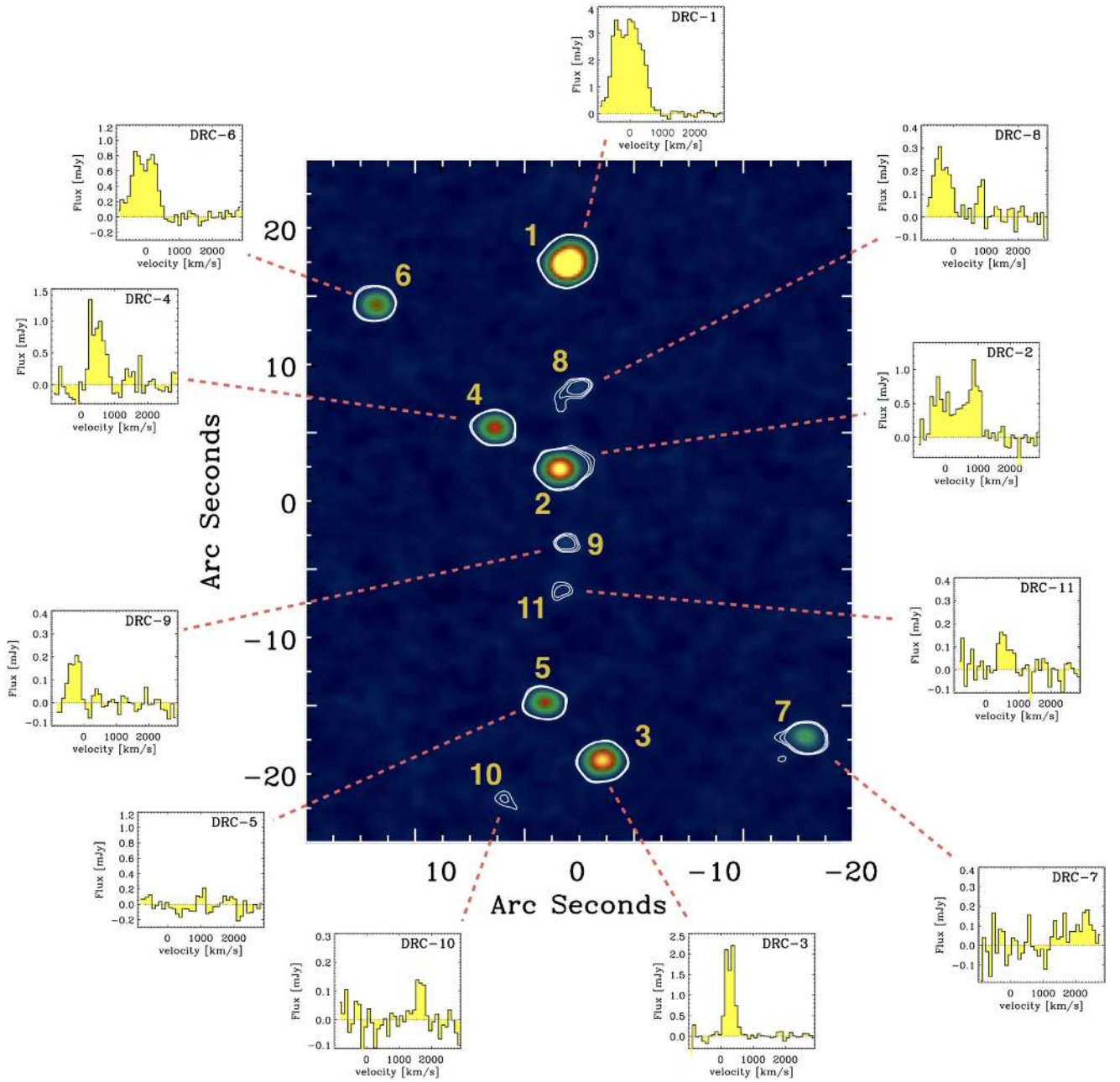
Figure 2. Spectroscopic confirmation of the protocluster members at z_{\text{spec}} = 4.002 via detection of ^{12}\text{CO}(6-5) emission (additional [\text{C I}](1-0) , \text{H}_2\text{O}(2_{11}-2_{02}) , ^{12}\text{CO}(4-3) and ^{12}\text{CO}(2-1) detections are shown in Figures 3–5). We have considered that the redshift of the structure corresponds to the redshift of DRC-1, its brightest component. The central panel shows the same 2 mm ultra-deep continuum imaging already shown in the central panel of Figure 1. The ^{12}\text{CO}(6-5) detections confirm that at least 10 of the 11 continuum sources belong to the protocluster. The lack of ^{12}\text{CO}(6-5) emission in DRC-5 does not necessarily mean that it does not belong to the protocluster, because the spectral setup of our ALMA observations does not cover velocities, v < -1000 \text{ km s}^{-1} . There is a wide range of line profiles, from relatively narrow emission (DRC-10) to extremely broad lines, as wide as \sim 1000 \text{ km s}^{-1} (DRC-1) or \sim 2100 \text{ km s}^{-1} (DRC-2). Note that the horizontal axes are not centered at v = 0 \text{ km s}^{-1} because the spectral setup of the ALMA observations only covers v > -1000 \text{ km s}^{-1} .
