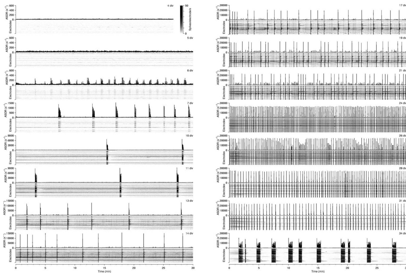
Figure 1 Development of burst patterns in a dense culture. Graphs show array-wide spike detection rates (ASDR) per second in recordings from one culture at various ages ( numbers in top right corners ). Note the different vertical scales used for each day. The spike detection rate of individual electrodes is represented by gray-scale rasters for all 59 electrodes, stacked vertically below each graph. (Each horizontal line pertains to one electrode; gray levels indicate firing rates. The same scale (see color bar next to '4 div') is used for all days. Note that the extreme increase in ASDR during bursts commonly saturates the gray scale. This representation is also used in subsequent figures.) Analogous figures from all 58 cultures used are available online.
