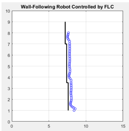
Figure 12. The Performance of WFR Controlled by FLC
