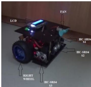
Figure 2. Wheeled Mobile Robot
