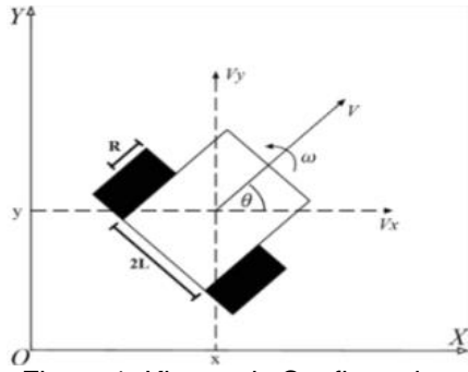
Figure 1. Kinematic Configuration
