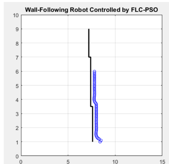
Figure 13. The Performance of WFR Controlled by FLC-PSO
