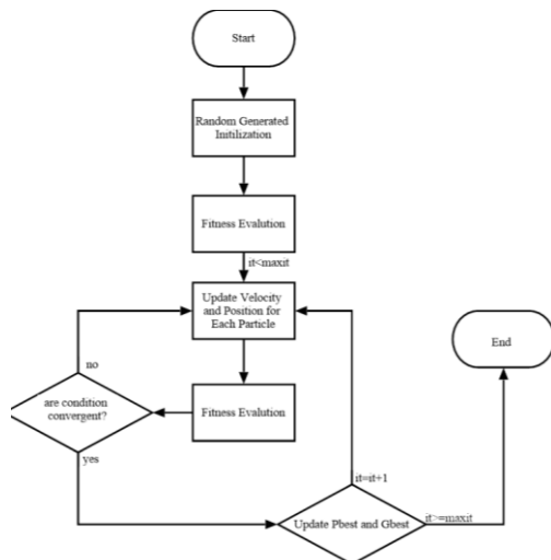
Figure 8. PSO's Flowchart
