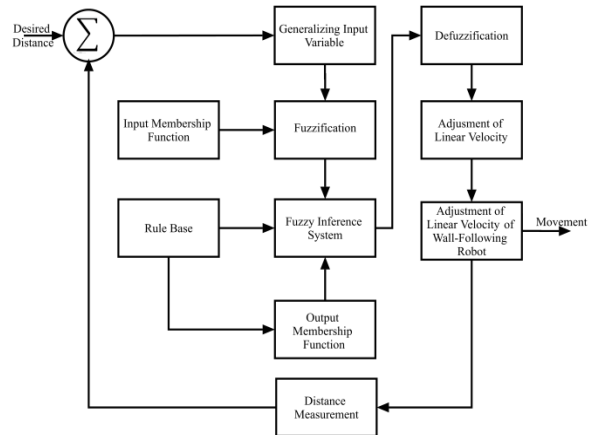
Figure 4. Flowchart of FLC for WFR
