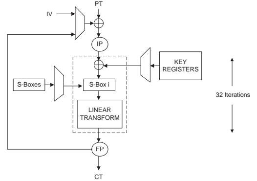
Figure 2: Iterative looping architecture block diagram
