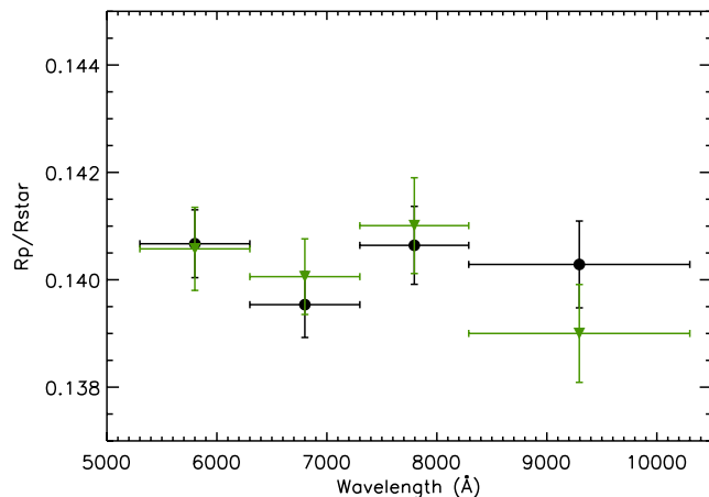
Figure 8. STIS G750L transmission spectrum of WASP-19b. The fits were performed using photon noise uncertainties on the data points, and then the error bars from MPFIT were rescaled with \beta_w , since we do not detect any red noise. The black points show the spectrum extracted using 3.75\sigma clipping in the cosmic ray removal routine, and green points show the spectrum extracted using 5\sigma clipping of cosmic rays.
