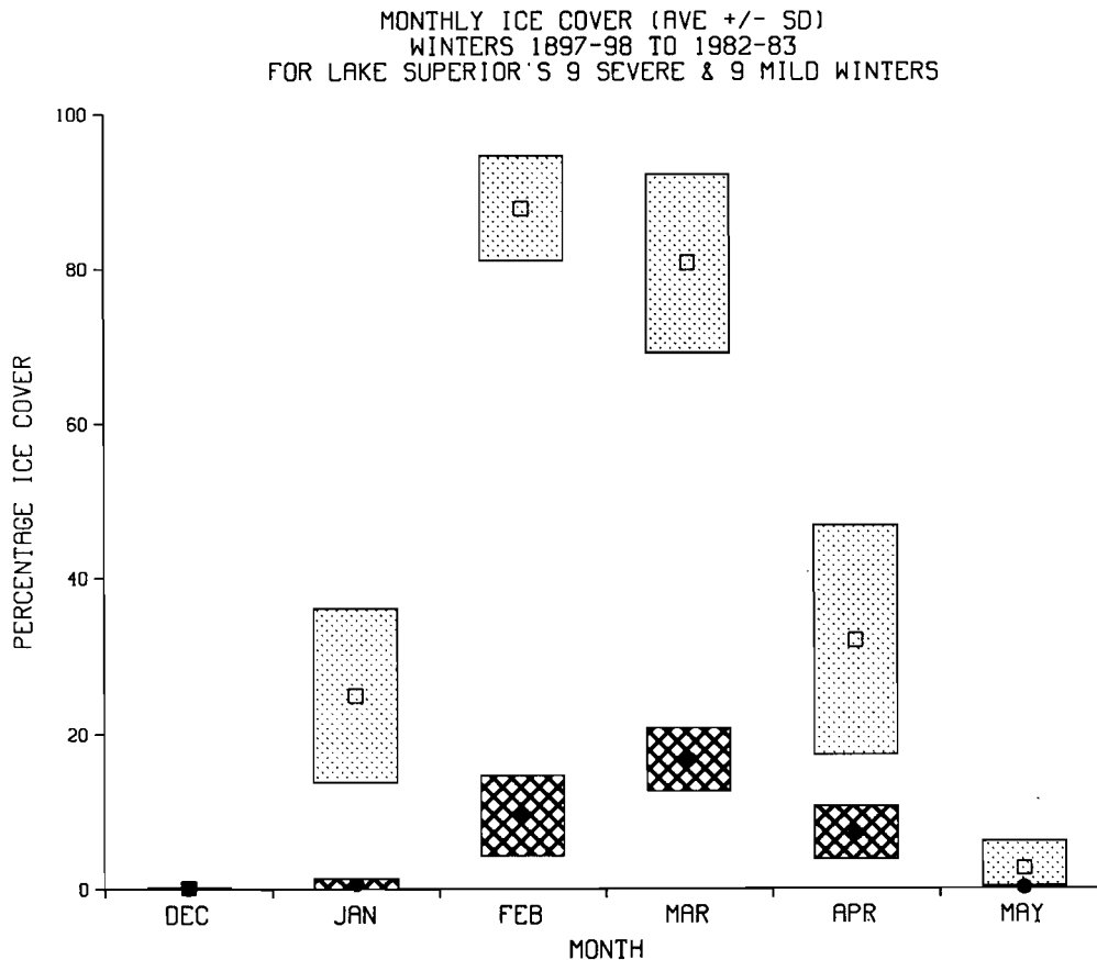
Figure 4. Reconstructed average monthly ice cover for mild winters (filled circles) and severe winters (open squares) for (a) Lake Superior and (b) Lake Erie. The hatched areas (mild winters) and stippled areas (severe winters) above and below the monthly average represent the variation over the nine winters (average plus and minus one standard deviation)
