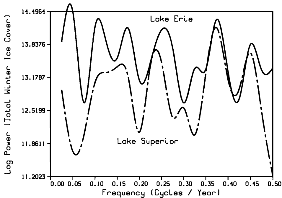
Figure 6. Spectral analysis of total winter ice cover for Lakes Superior and Erie, using the Daniell spectral window with the spectral window smooth parameter M set to 40
