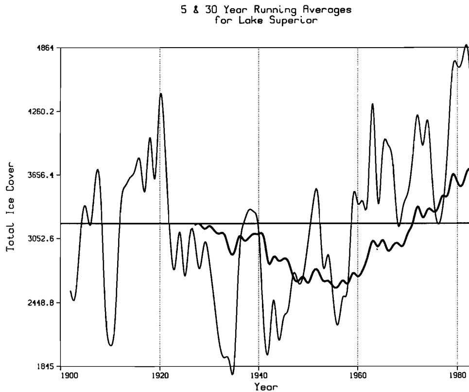
Figure 5. Equally weighted 30-year continuous (thick solid line) and 5-year continuous (thinner solid line) averages of the reconstructed total winter ice cover for (a) Lake Superior and (b) Lake Erie. The heavy horizontal line on each graph is the long-term (86 winter) average. The 30-year and 5-year continuous averages are plotted on the year they end; for example, the first 30-year continuous average is calculated for the years 1898–1927 and is plotted on the year 1927
