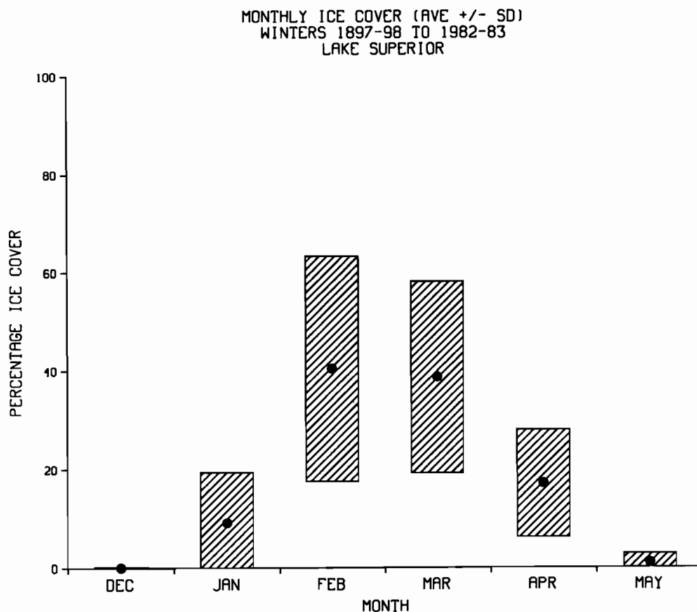
Figure 2. Reconstructed long-term (86-winter) average monthly ice cover (filled circle) plus and minus one standard deviation (hatched area): (a) for Lake Superior and (b) for Lake Erie
