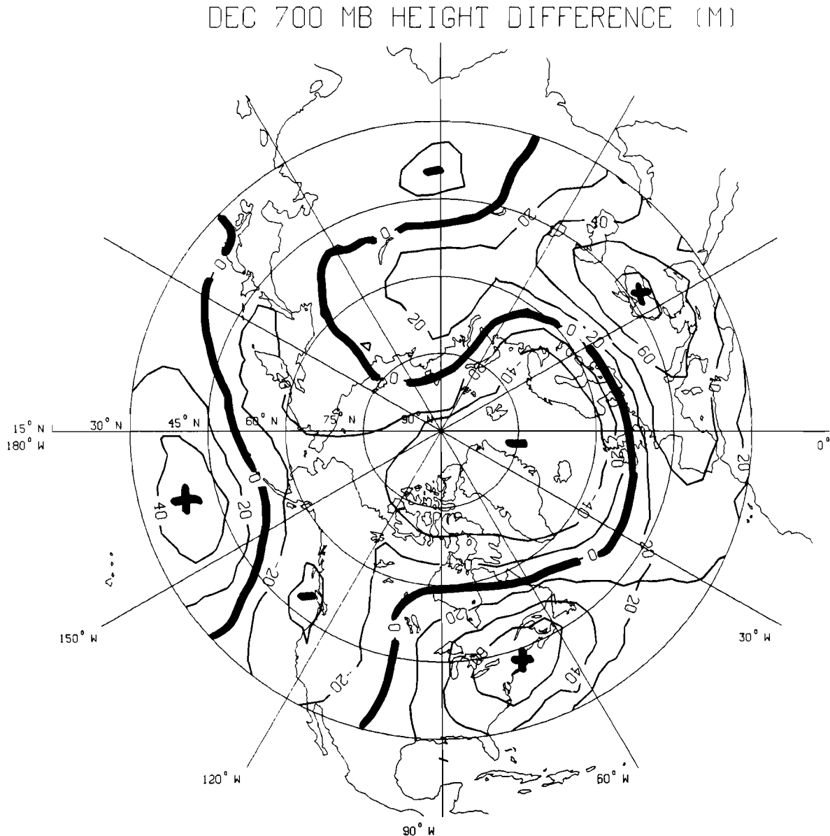
Figure 3. Contour analysis of: monthly 700-mbar heights averaged for the mild ice seasons (1948–1949, 1949–1950, 1952–1953, 1972–1973, and 1982–1983) minus monthly 700-mbar heights averaged for the severe ice seasons (1958–1959, 1962–1963, 1969–1970, 1977–1978, 1978–1979, and 1981–1982) for (a) December, (b) January, and (c) February. The contour interval is 10 m. Pluses and minuses show the centres of maximal positive and negative differences
