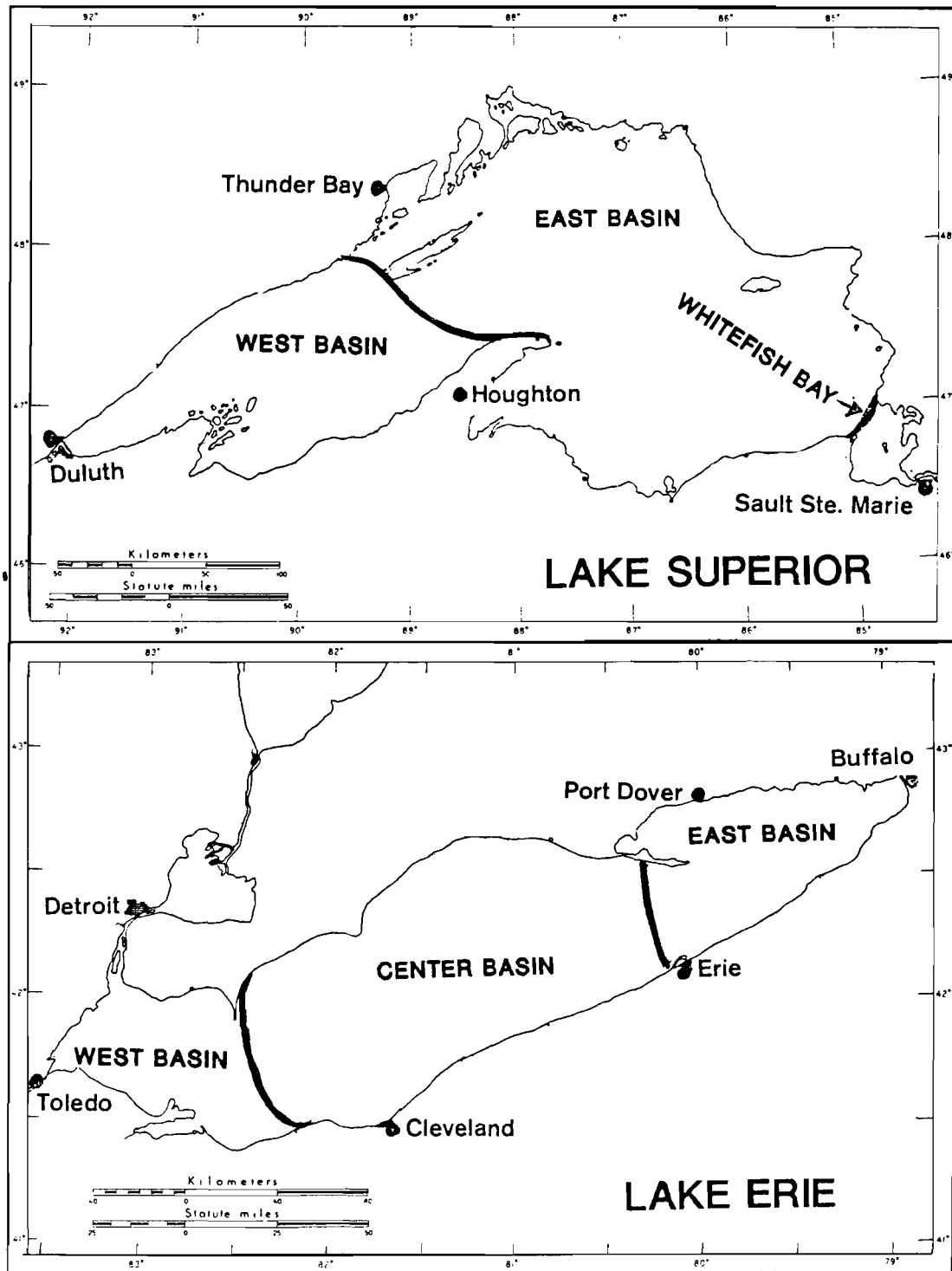
Figure 1. East, west, and Whitefish Bay basins of Lake Superior and east, central, and west basins of Lake Erie used in ice-cover models. Air temperature stations used for FDD analysis (see Tables I and III)
