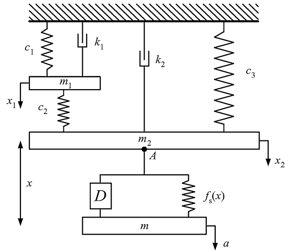
Fig. 7 Schematic of system used in simulation studies
