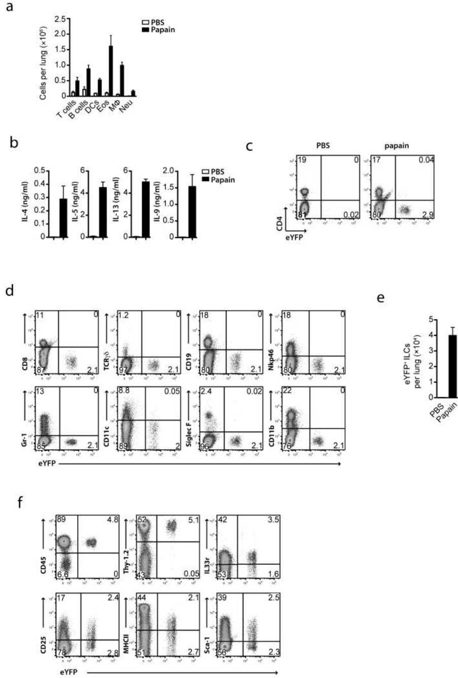
Figure 1. Papain induced eYFP + cells do not express any lineage markers (a) Number of cells in the lungs of IL9 Cre R26R eYFP mice challenged with papain (black bars) and PBS (white bars) on days 0, 3, 6, 14 and analysed 20 h after the last re-challenge (see scheme Supplementary Fig.9). (b) Cytokine concentration in the broncho-alveolar lavage fluid (BALF) of mice immunized with papain (black bars) or PBS (white bars) as in a . (c,d) Flow cytometry of total lung cells from papain challenged IL9 Cre R26R eYFP mice as in a stained for CD4 (c) or TCR \beta , CD8 \alpha , TCR \gamma\delta , CD19, Nkp46, Gr-1, CD11c, SiglecF and CD11b (d) and assessed for eYFP expression. (e) Absolute number of eYFP + ILC in the lung of papain challenged IL9 Cre R26R eYFP mice. (f) Flow cytometry of CD45, Thy1.2,
