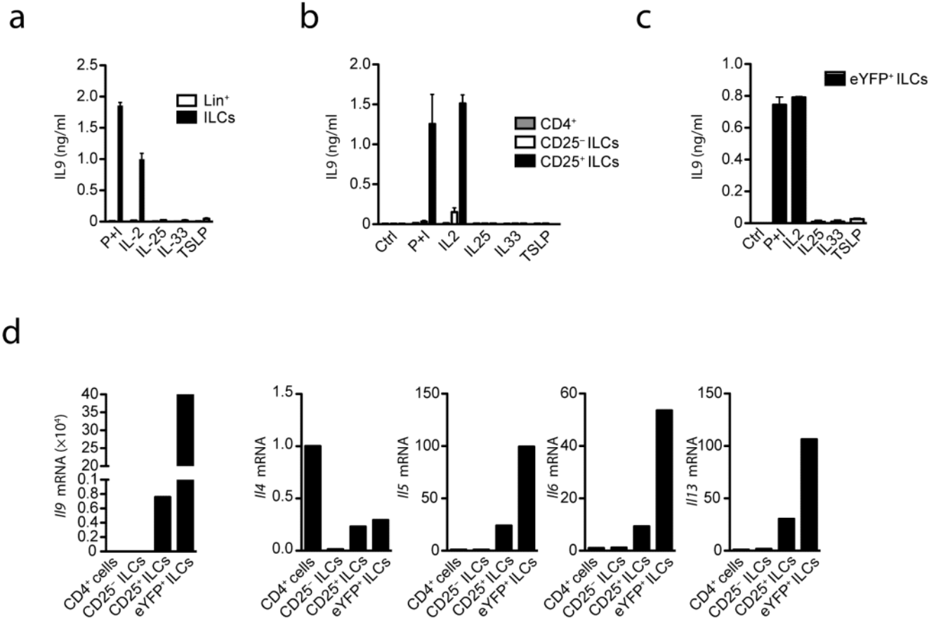
Figure 3. IL-9 in ILC is induced by IL-2 but not IL-25, IL-33 or TSLP
