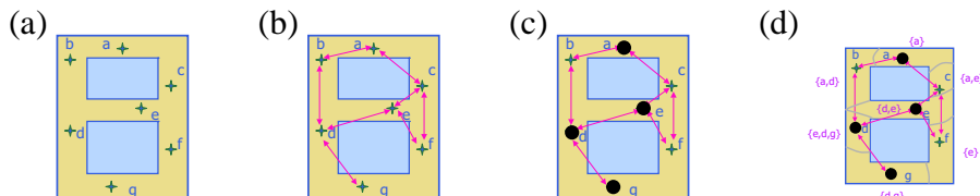
Fig. 1. Our location detection system. (a) Discrete locations. (b) Connectivity. (c) Beacon placements. (d) Covering regions of each discrete point and corresponding identifying sets.
