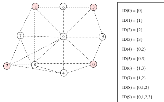
Fig. 3. The connectivity graph of the testbed and its identifying codes. The filled dots denote the positions that transmitters are placed.
