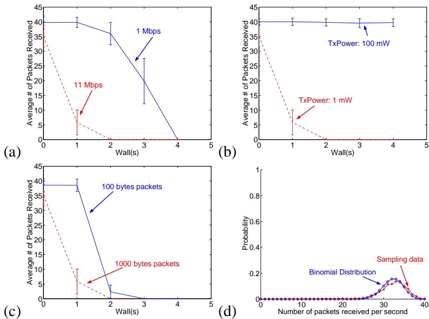
Fig. 2. Reception Range versus (a) data rates, (b) transmitting power, (c) packet size and (d) packet arrival rate distribution
