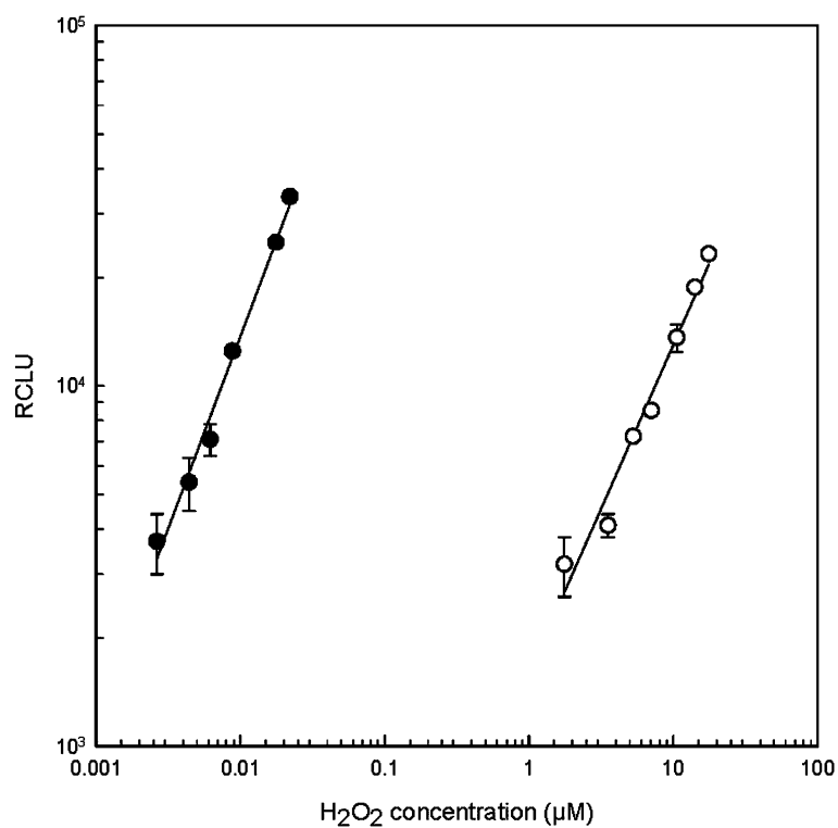
Figure 1. Determination of H 2 O 2 by the chemiluminescence of luminol catalysed either by ferricyanide (○) or Co (II) (●). Values for H 2 O 2 concentration are placed in logarithmic scale to remark the differences between catalyst. RCLU (relative chemiluminescence units).
