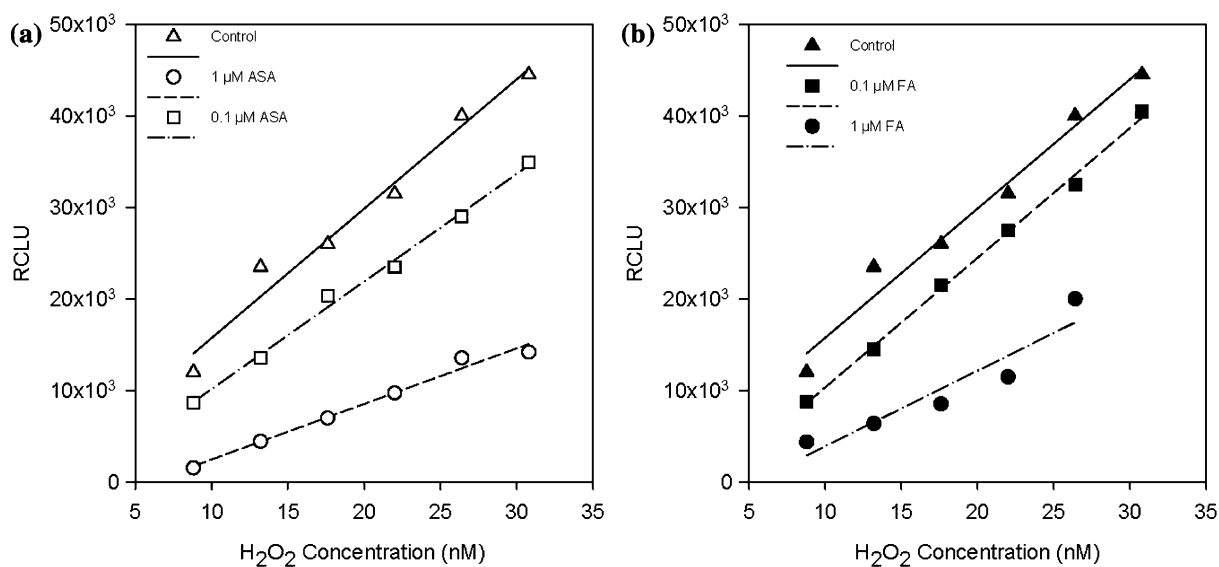
Figure 2. Quenching effect of ascorbic ASA (a) and ferulic acid (b) on the chemiluminescence of luminol catalysed by Co (II) in the presence of different concentration of H 2 O 2 . The concentration of quencher was 1 (○) and 0.1 μM (□). RCLU (relative chemiluminescence units).
