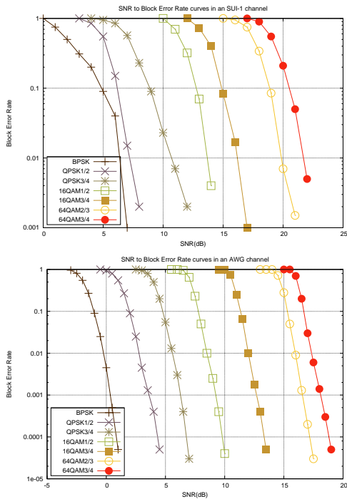
Figure 2: SNR to Block Error Rate curves in a SUI-1 and AWGN channels.
