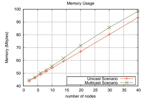
Figure 9: Memory required vs. number of nodes.
