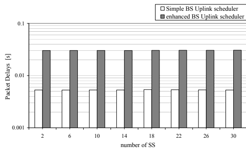
Figure 6: Packet latency vs. number of SSs.
