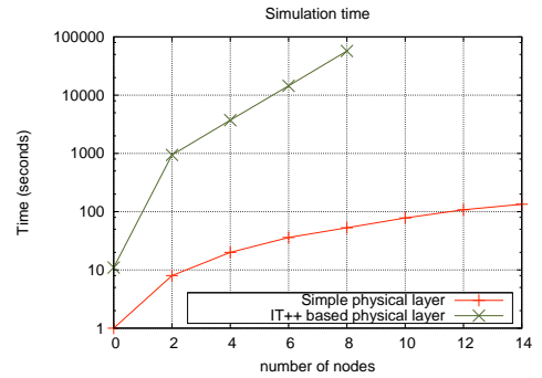
Figure 1: Time needed to execute a WiMAX scenario of 5 second while varying the number of SS.
