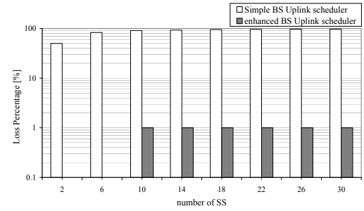
Figure 4: Packet Loss Ratio vs. number of SSs.
