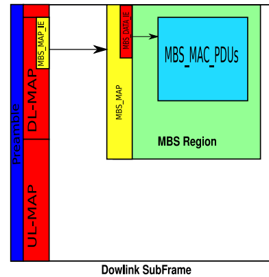
Figure 7: DL sub-frame structure with MBS zone.
