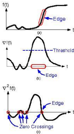
Fig. 1. (a)Original imagesignal (one-dimension); (b)Gradientoftheoriginal imagesignal (firstderivativewithrespecttot); (c)Laplacianoperationonthe originalsignal (second derivative with respect to t)
