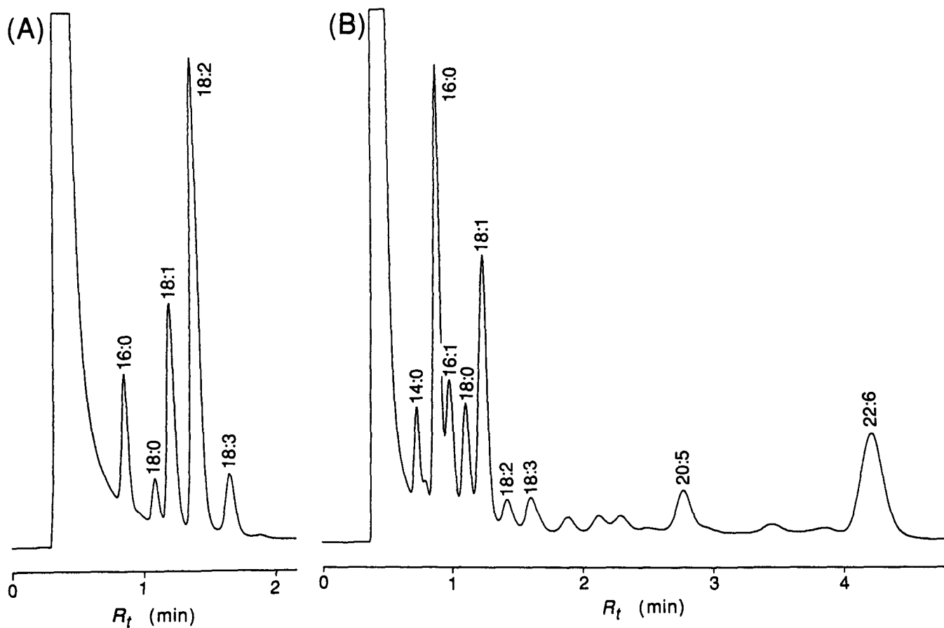
FIG. 5. High-speed gas chromatography (GC) of fatty acid methyl esters prepared from (A) soybean oil and (B) a 22:6-enriched fish oil. GC conditions: 3 mm \times 2 m glass column; column packing, 10% SP-2340 on 100–120 mesh Chromosorb WAW; column temperature, 240°C; N_2 , 40 mL/min.
