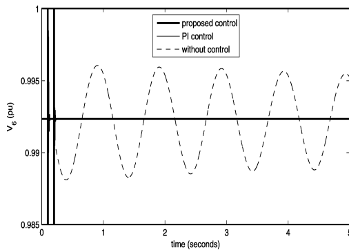
Fig. 8. Voltage magnitude at bus 6—Case I.
