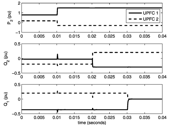
Fig. 19. Active and reactive UPFC powers—Case V.
