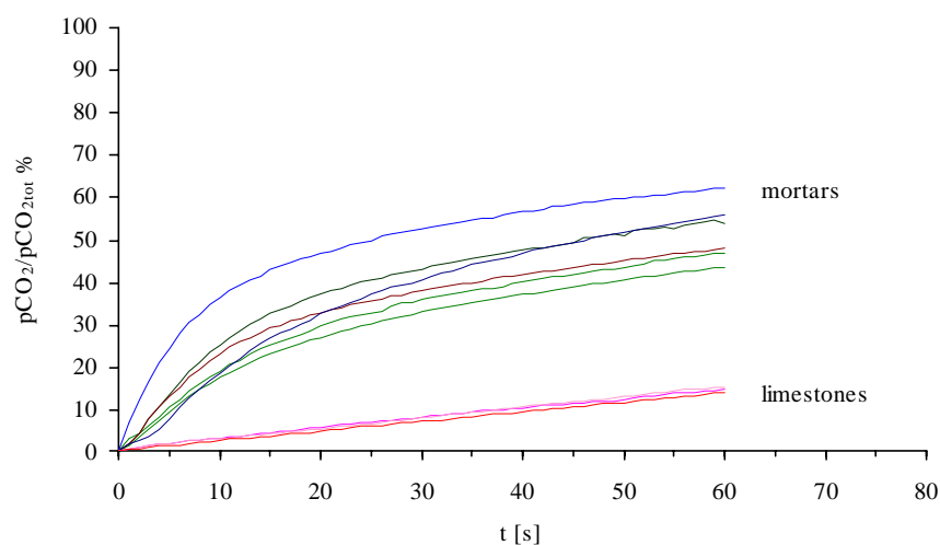
Figure 1 The CO 2 yield as a function of time for six mortar and four fossil limestone carbonates. The CO 2 pressure recorded is given relative to the maximum reached at the end of reaction. The grain size range is 43–62 microns.
