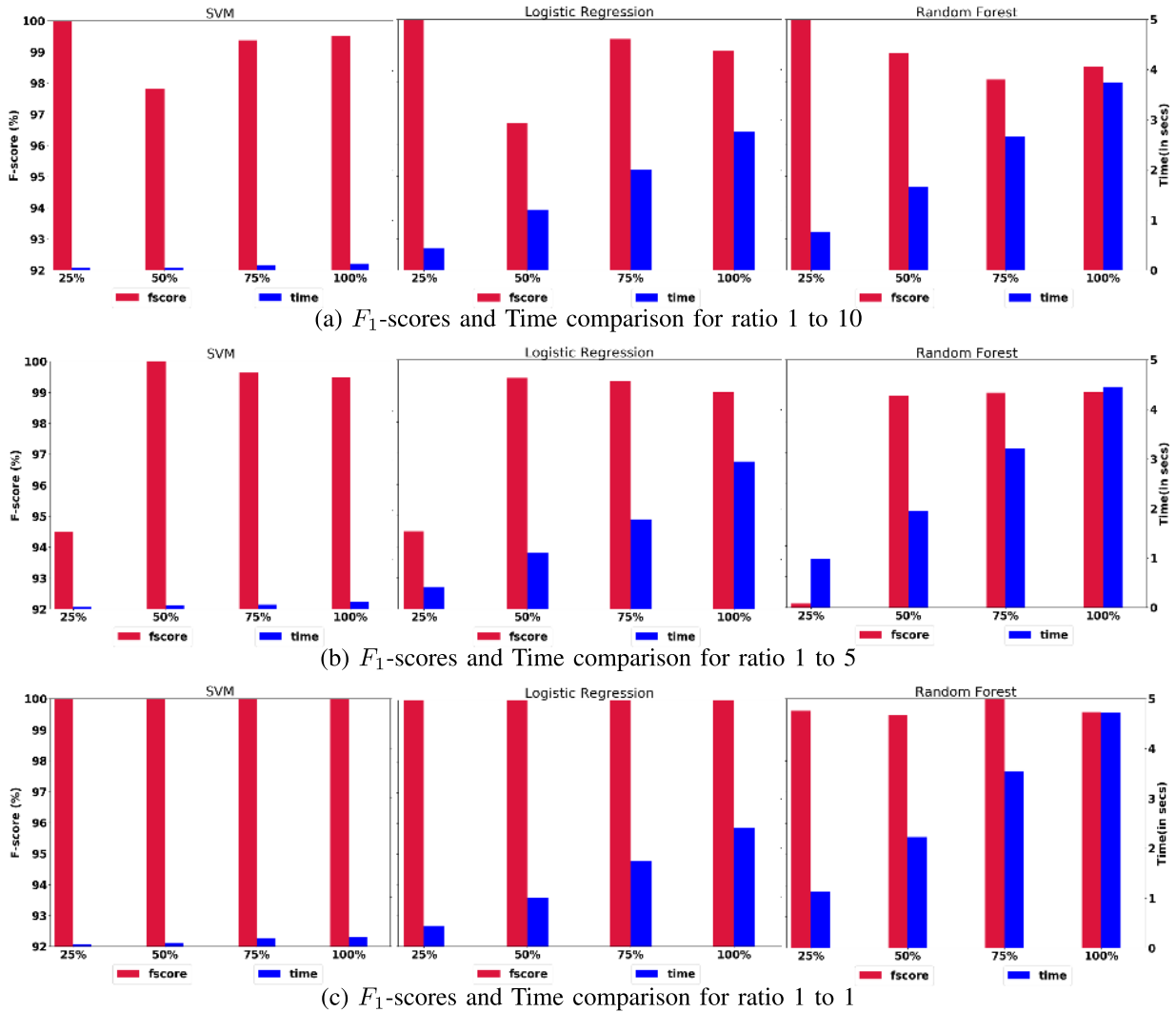
FIGURE 8. Scaling performance of top classifiers on emails with header on three ratios 1:1, 1:5, and 1:10.
