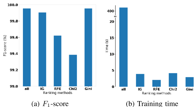
FIGURE 11. Comparison of performance of top classifier with all features vs top 20 features for Emails - with header features.
