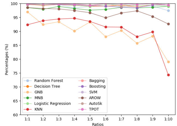
(a) With Header Features
