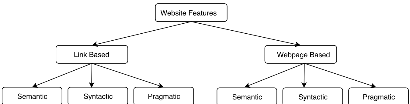
FIGURE 1. URL and Website feature taxonomy. Each category at the bottom level is a subtree which consists of the finer feature categories - Lexical, Network and Script further described in Section IV-B.
