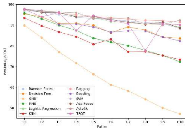
FIGURE 5. Changes in F_1 -score Performance with varying ratios between legitimate and phishing URLs.
