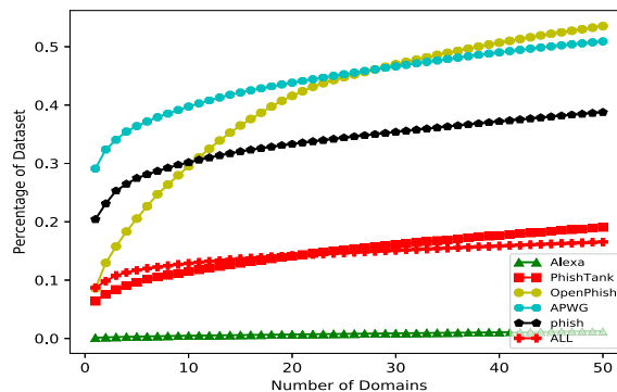
(a) CDF of top 50 Domains in each dataset separately and all datasets combined
