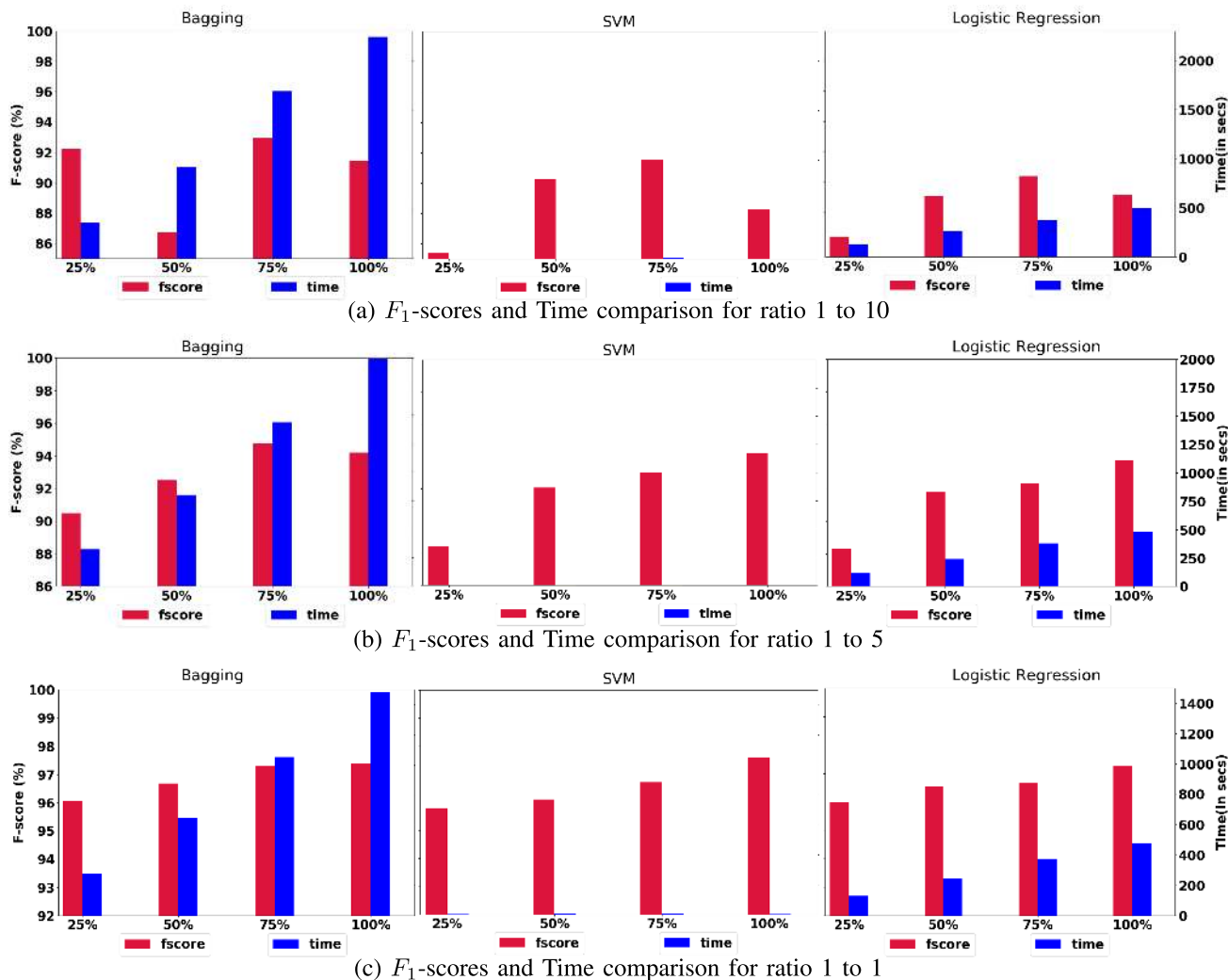
FIGURE 7. Scaling performance of top classifiers on websites on three ratios 1:1, 1:5, and 1:10.
