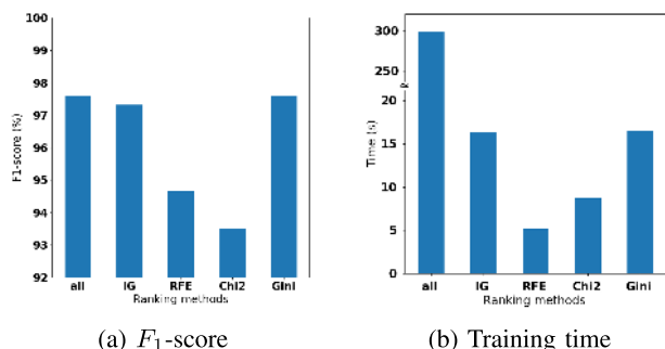
FIGURE 10. Comparison of performance of top classifier with all features vs top 20 features for websites.
