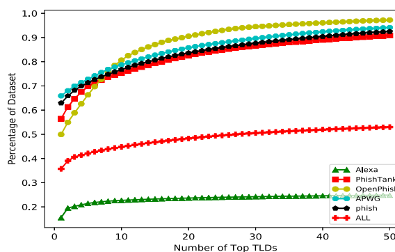
(b) CDF of top 50 TLDs in each dataset separately and all datasets combined
