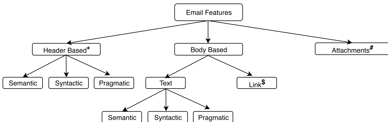
FIGURE 2. Email feature taxonomy. Each category at the bottom level is a subtree which consists of the finer feature categories - Lexical, Network and Script further described in Section IV-C. * Script-based features cannot be extracted from email headers. $ Please see the subtree on Link Based features under the Website taxonomy. # Attachment features have been described in Section IV-C.
