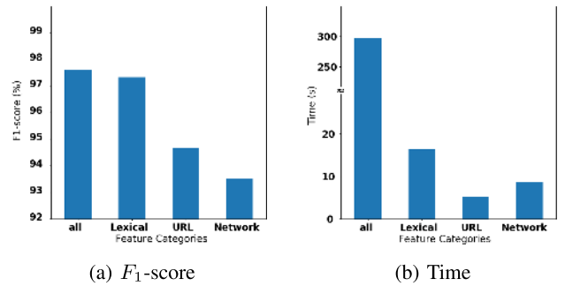
FIGURE 13. Comparison of the performance of top classifier with all features vs features from each category of websites features.
