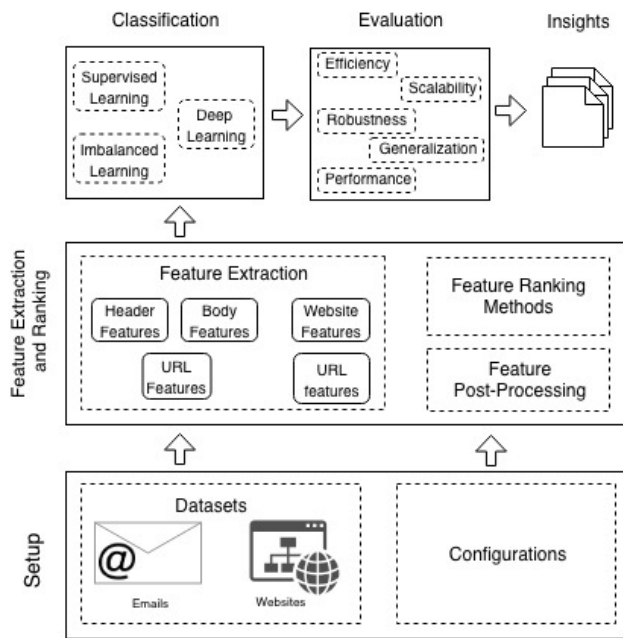
FIGURE 3. Schema of proposed benchmarking framework and system evaluation for phishing.
