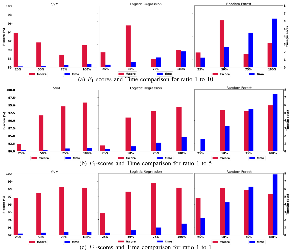
FIGURE 9. Scaling performance of top classifiers on emails with no header on three ratios 1:1, 1:5, and 1:10.
