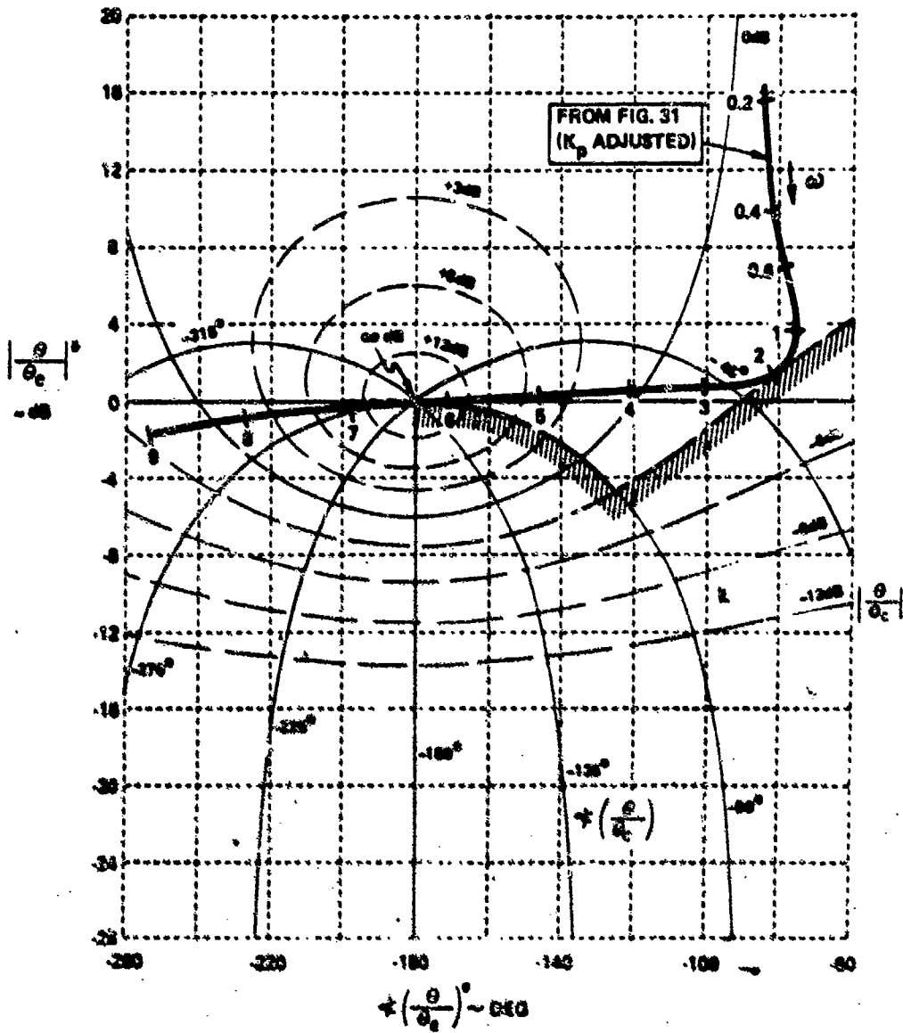
Figure 32. Overlay of |\theta/\theta_c|^2 Versus \angle(\theta/\theta_c)^\circ on a Nichols Chart (Configuration with High \omega_{3r} )
