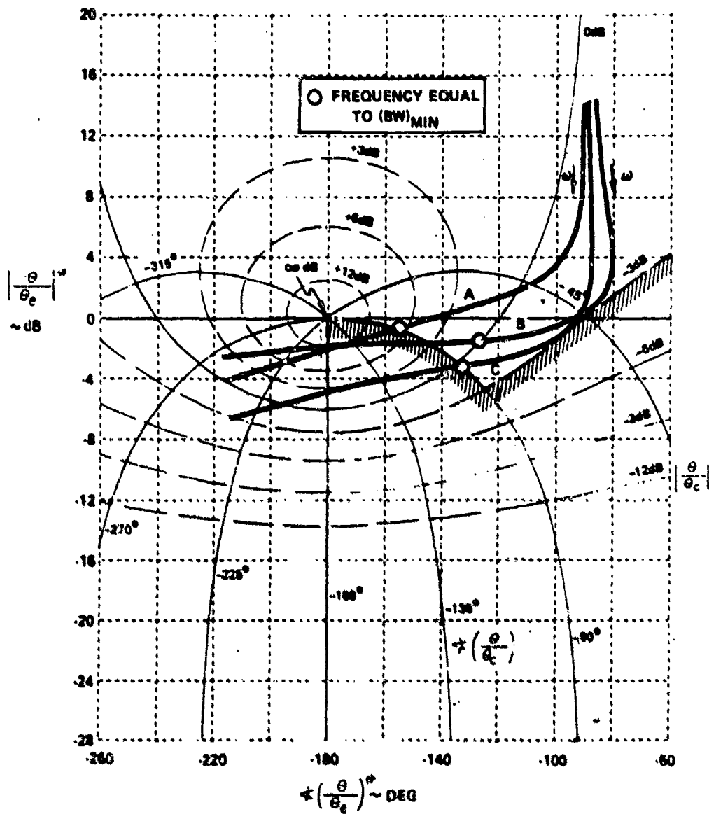
Figure 21. Typical Overlays of \left| \theta / \theta_c \right|^2 Versus \angle \left( \theta / \theta_c \right) on a Nichols Chart
