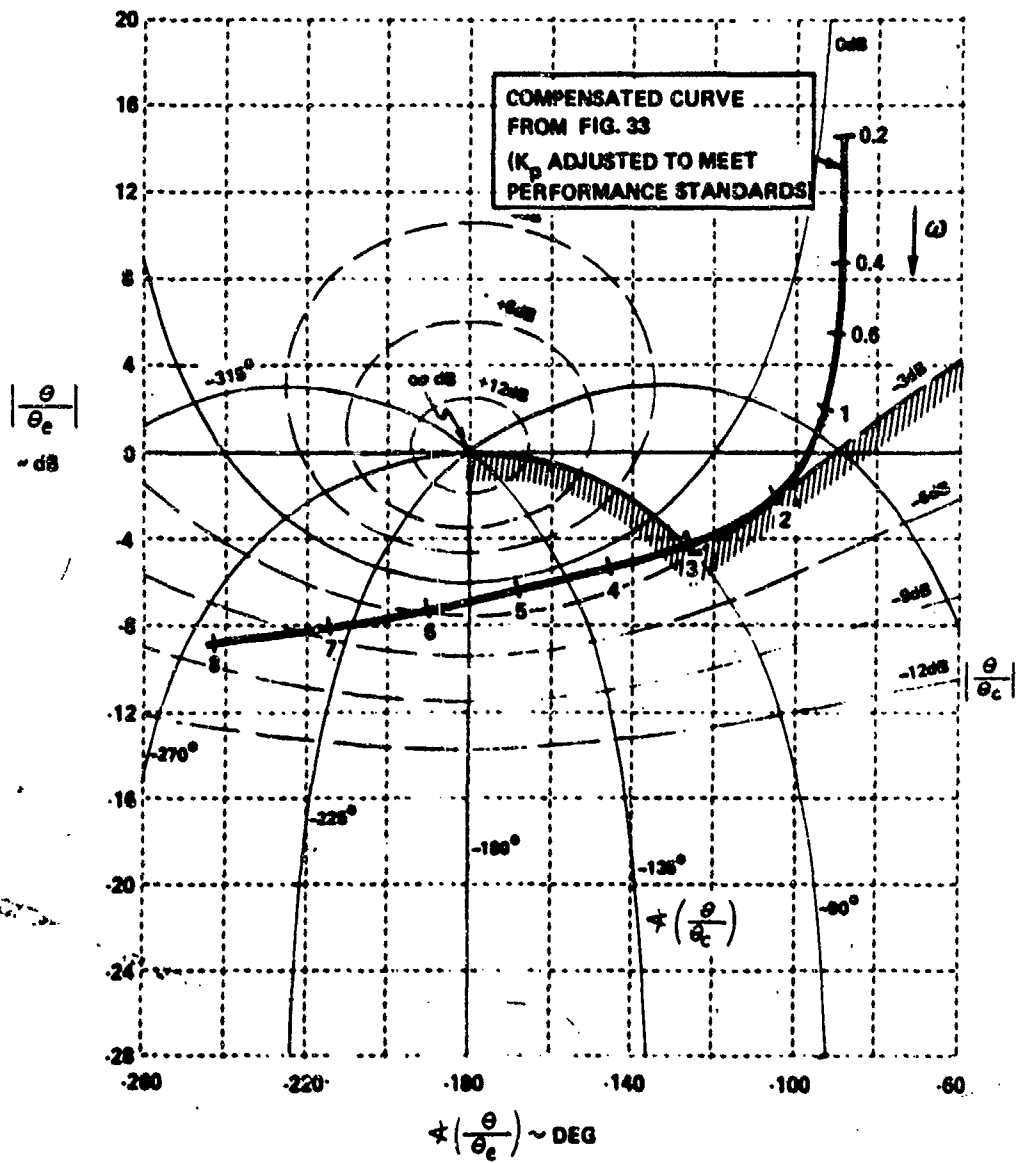
Figure 34. Lag-Compensated Amplitude-Phase Curve Overlaid on a Nichols Chart (Configuration with High \omega_{sp} )
