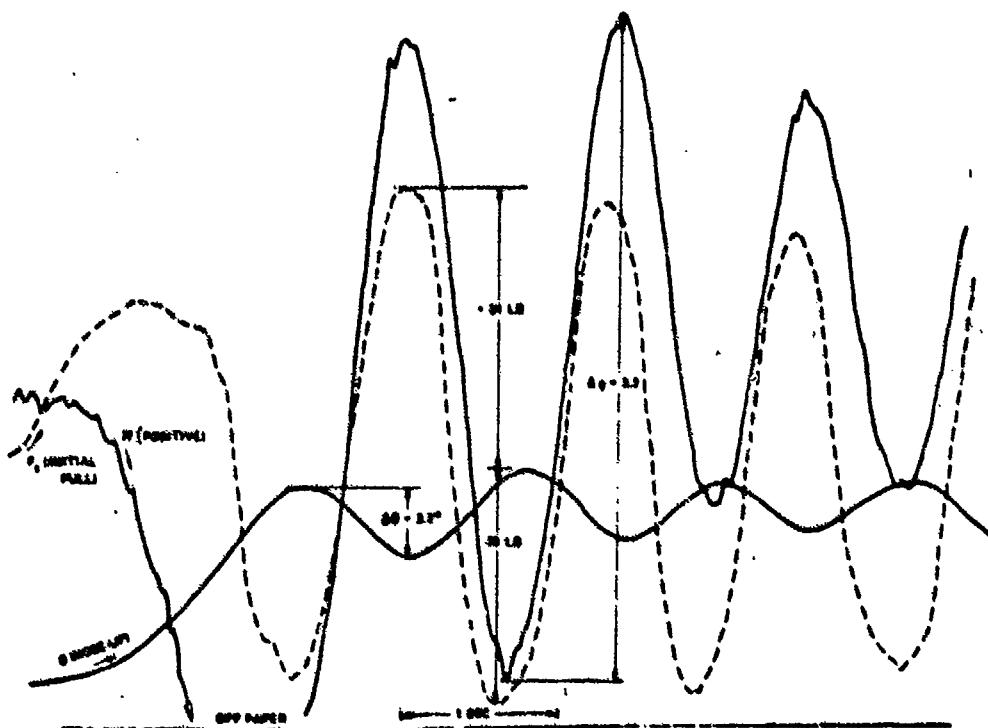
Figure 41. In-Flight Record of a PIO Occurring During Visual Tracking (Configuration 6E, Flight 1071)
