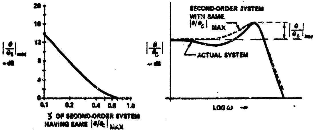
Figure 37. Damping Ratio of Simple Second-Order System as a Function of |\theta/\theta_c|_{\max}
