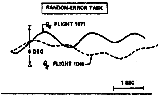
Figure 36. Typical IFR Tracking Records for Configuration 6E
