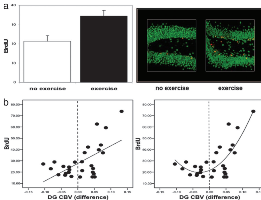
Fig. 2. Exercise-induced increases in dentate gyrus CBV correlate with neurogenesis. (a) (Left) Exercising mice were found to have more BrdU labeling compared with the no-exercise group. (Right) As shown by confocal microscopy, the majority of the new cells were colabeled with NeuN (red, BrdU labeling; green, NeuN; yellow, BrdU/NeuN double labeling). (b) (Left) A significant linear relationship was found between changes in dentate gyrus CBV and BrdU labeling. (Right) A quadratic relationship better fits the data. The vertical stippled line in each plot splits the x axis into CBV changes that decreased (left of line) versus those that increased (right of line) with exercise.
