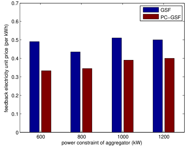
Fig. 7: Impact on feedback electricity unit prices when four aggregators have different power constraints
