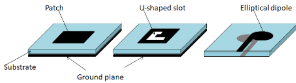
FIGURE 10. Different types of microstrip antennas; (a) rectangular patch antenna; (b) broadband patch antenna with u-shaped slot; (c) elliptical dipole antenna [128].
