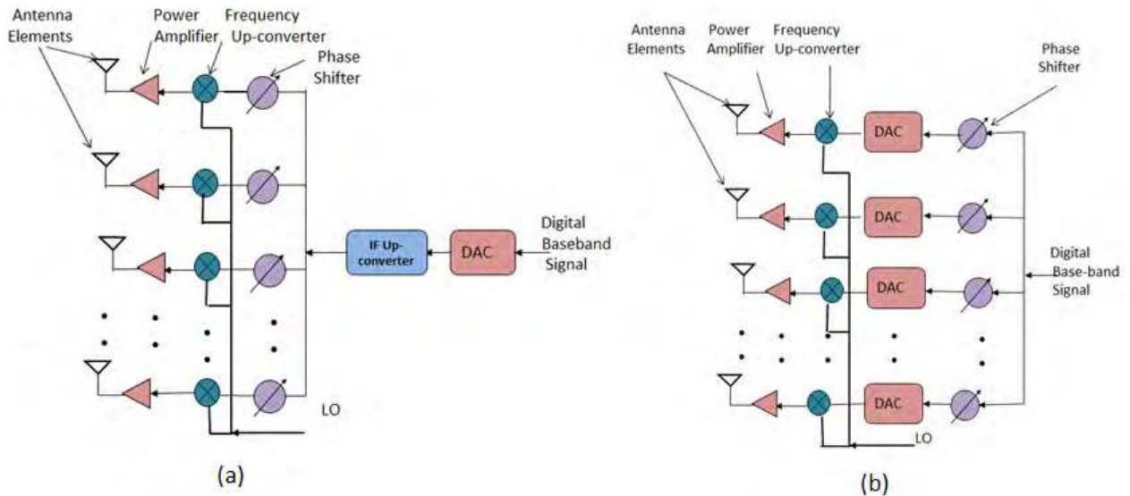
FIGURE 6. (a) Analog IF beam-forming; (b) digital beam-forming antenna array.
