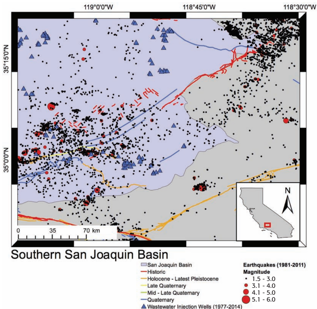
Figure 4.4-5. Earthquakes M \geq 1.5 in the southernmost San Joaquin Valley from Hauksson et al. (2012). Wells and faults as in Figure 4.4-4.
