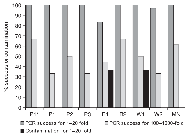
Fig. 1 Percentages of PCR success and contamination in a test of seven glass fibre plates (P1-3, B1-2, W1-2) and one commercial kit (MN). DNA was extracted from eight lysate concentrations from six mammal species. All plates were run using automation except P1*.
