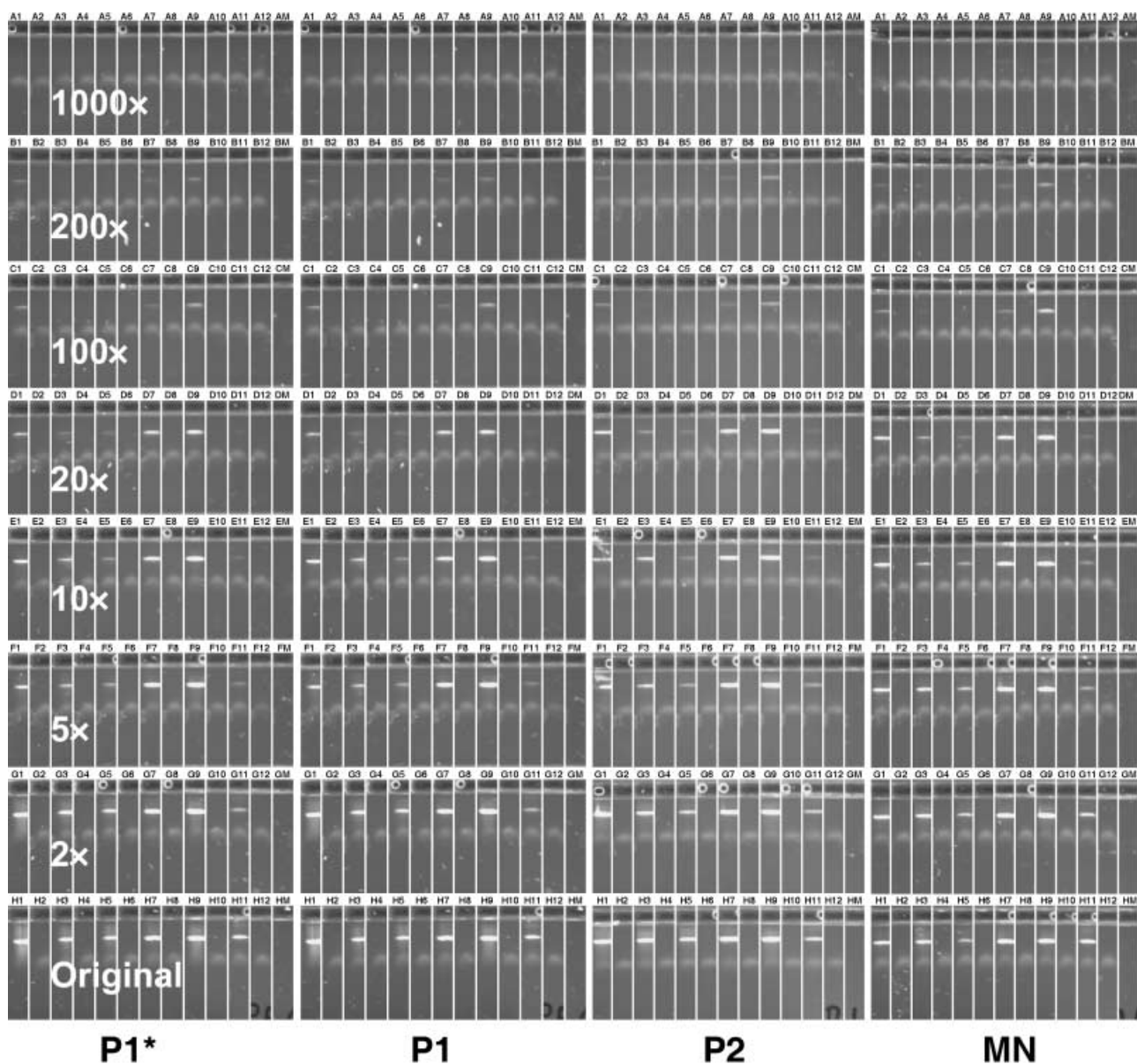
Fig. 2 PCR products (658 bp) for the COI (cytochrome c oxidase I) barcode region from DNA isolated using two glass fibre plates (P1, P2) and one commercial kit (MN) for 1–1000-fold dilutions of lysates from six mammal species. Except for P1*, results were obtained using automation. Some faint products are not visible in this agarose gel image. Even numbered lanes are negative controls.
