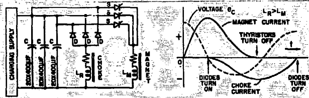
FIG. 2. CIRCUIT WITH CHARGE RECOVERY CHOKES AND ASSOCIATED WAVEFORMS. IF DIODES D ARE REPLACED WITH THYRISTORS THE WAVEFORMS OF FIG. 1 APPLY.
