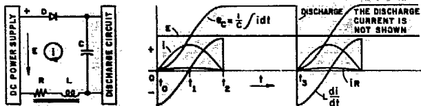
FIG. 5 CONVENTIONAL CHARGING CHOKE CIRCUIT AND ASSOCIATED WAVEFORMS
