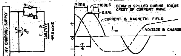
FIG. 1 CONVENTIONAL CAPACITOR DISCHARGE CIRCUIT AND ASSOCIATED WAVEFORMS
