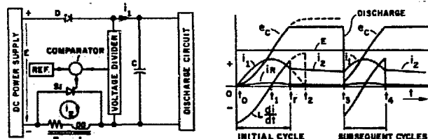
FIG. 6 CHARGING CHOKE CIRCUIT WITH TURN-OFF THYRISTOR AND ASSOCIATED WAVEFORMS
