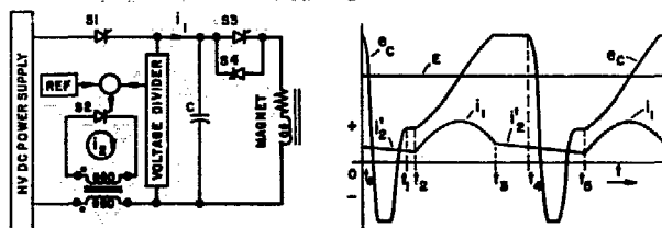
FIG. 7 REACTOR-TRANSFORMER CHARGING CIRCUIT WITH TURN-OFF THYRISTOR AND ASSOCIATED WAVEFORMS
