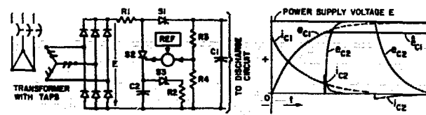
FIG. 4 CHARGING CIRCUIT WITH THYRISTOR TURN-OFF AND ASSOCIATED WAVEFORMS
