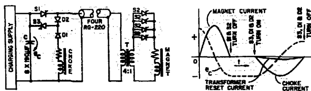
FIG. 3 DISCHARGE CIRCUIT WITH MATCHING TRANSFORMER AND ASSOCIATED WAVEFORMS
