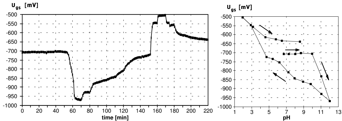
Figure 2. Dynamic response and calibration curve to pH of an ISFET with polyHEMA coating deposited according to the Method 2, with subsequently increased thickness by dropping of additional portion of HEMA by means of micropipette. Cycle of pH changes: 6.5-12-2-8.5.
