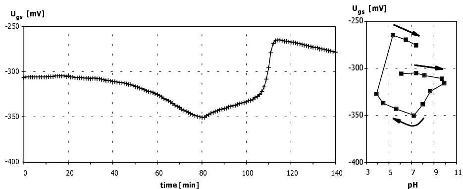
Figure 5. Dynamic response and calibration curve to pH of an ISFET with polyHEMA coating ca. 60 \mu\text{m} thick, deposited according to the Method 3. Cycle of pH changes: 6-10-4-7.
