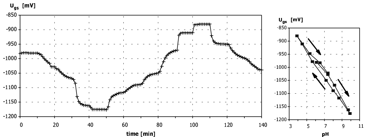
Figure 4. Dynamic response and calibration curve to pH of an ISFET with polyHEMA coating ca. 20 \mu\text{m} thick, deposited according to the Method 3. Cycle of pH changes: 6-10-4-7.
