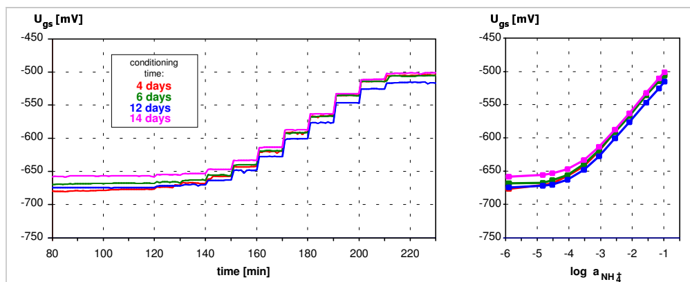
Figure 8. Dynamic responses and calibration curves of an ammonium ion sensor with membrane of Siloprene K 1000, fabricated on ISFET structure with silicon nitride gate insulator.
