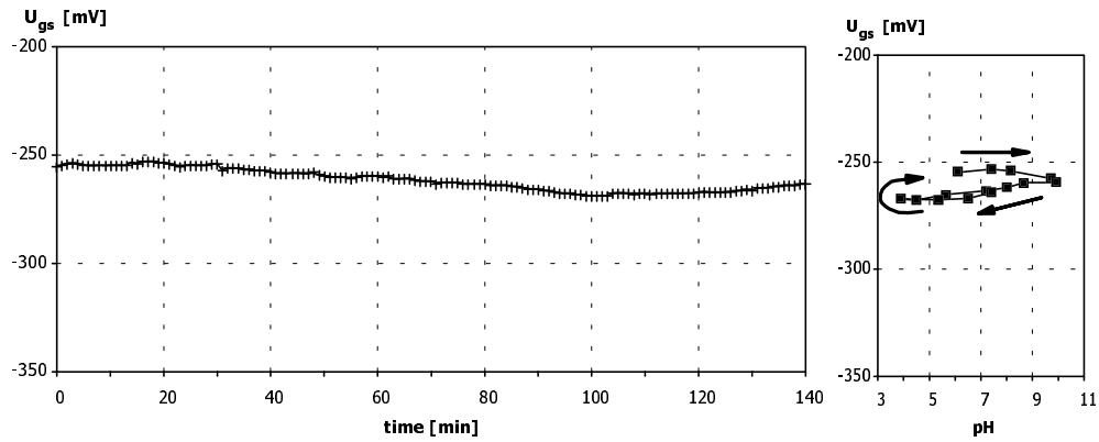
Figure 6. Dynamic response and calibration curve to pH of an ISFET with polyHEMA coating ca. 100 \mu\text{m} thick, deposited according to the Method 3. Cycle of pH changes: 6-10-4-7.
