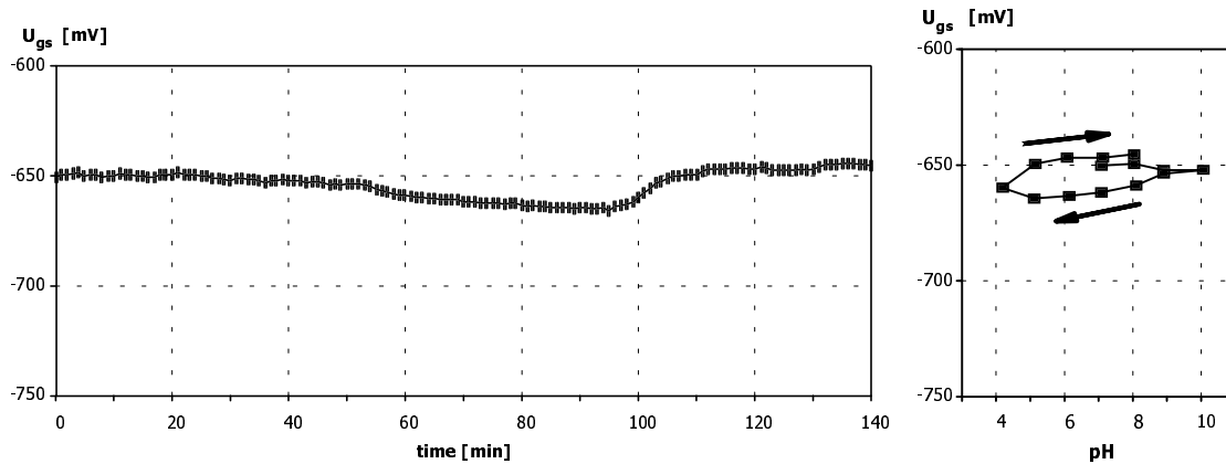
Figure 3. Dynamic response and calibration curve to pH of an ISFET with polyHEMA coating deposited according to the Method 2, with subsequently increased thickness by dropping of additional portion of HEMA cocktail by means of micropipette. Cycle of pH changes: 7-10-4-8. (Measurements performed for the same ISFET as in Fig. 3, but in restricted pH-range).
