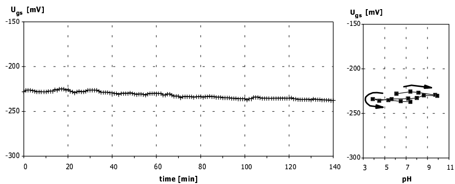
Figure 7. Dynamic response and calibration curve to pH of an ISFET with polyHEMA coating ca. 160 \mu\text{m} thick, deposited according to the Method 3. Cycle of pH changes: 6-10-4-7.
