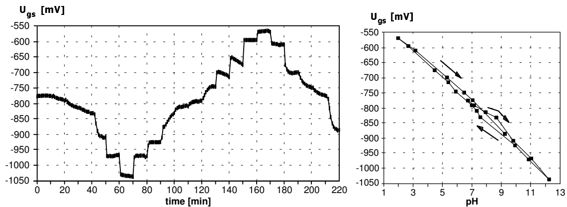
Figure 1. Response to pH changes of an ISFET with polyHEMA coating deposited according to the Method 2. Cycle of pH changes: 7-12-2-9.
