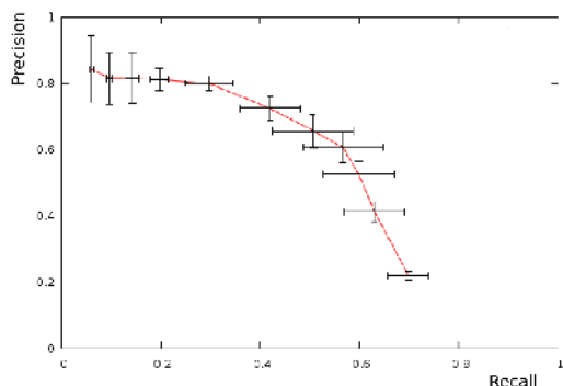
Figure 3. Recall/Precision for a 10 word lexicon on the RIMES database
