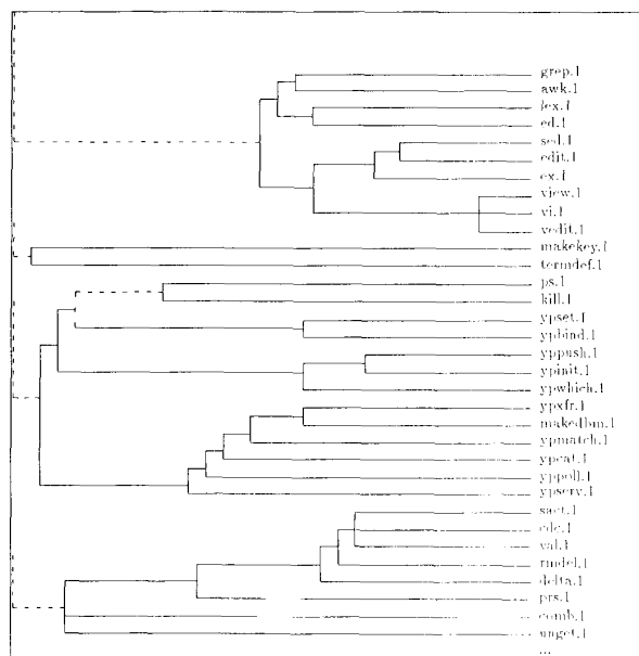
Fig. 4. Portion of AIX hierarchy (single link, k = 0.5 ).
