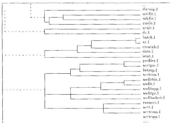
Fig. 5. Portion of AIX hierarchy (single link, k = 0.5 ).
