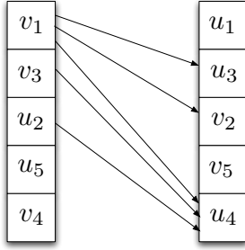
Fig. 3. One of the several 5 \times 2 tables generated by running algorithm \mathcal{P} on the \mathcal{G}_c, \mathcal{G}_r shown in Fig. 2. The order of choosing sinks was v_4, u_5, u_2, v_3, u_4, u_3, v_2, v_1, u_1, v_5 . The arrows show connectivity from the vertices on the left to the vertices on the right in \mathcal{G}_c . Note that arrows never go ‘horizontally’ or ‘upward’ but only go ‘downward’ which is the desired GNS-cut property.
