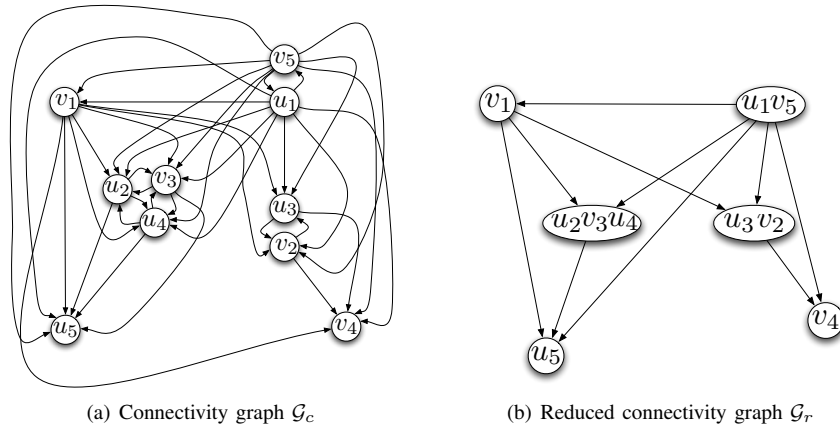
Fig. 2. Connectivity graph and reduced connectivity graph for an instance of a 5-pair unicast directed symmetric-demand network
