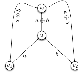
Fig. 1. All edges have unit capacity
