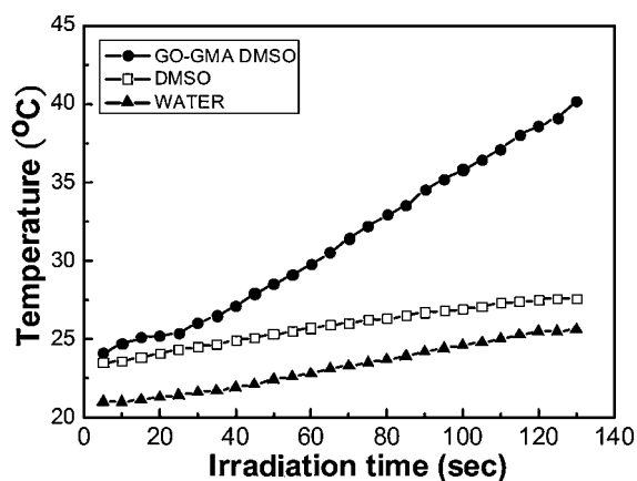
Fig. 5 Temperature response of GO–GMA upon IR light irradiation. The overall exposure duration is 2 min with power density of 1.2\text{ W cm}^{-2} .
