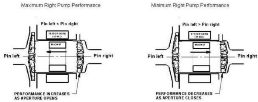
Figure 2. Atrial pressure differential effects on rotor position and right pump performance.
