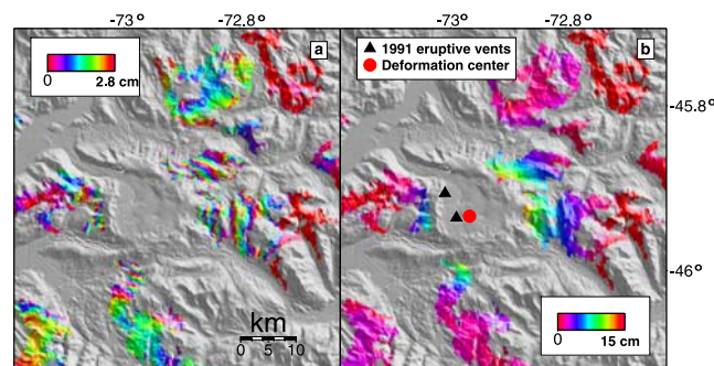
Figure 2. a. Wrapped interferogram at Cerro Hudson between 3 March 1996–22 February 1999. b. Unwrapped interferogram. The RMS difference between this data and a spherical model is 1.4 cm.
