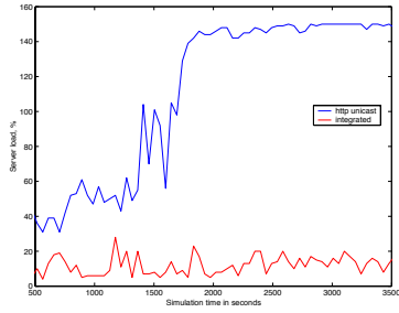
Figure 4. Server Load - Equal Delays between Clients Requests
