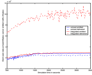
Figure 2. Increased Load Goodput: Transmitted data vs. Received data
