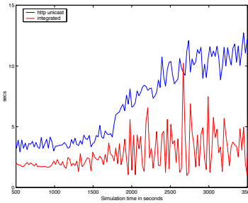
Figure 5. Client Seen Delay: pages 6 and 7
