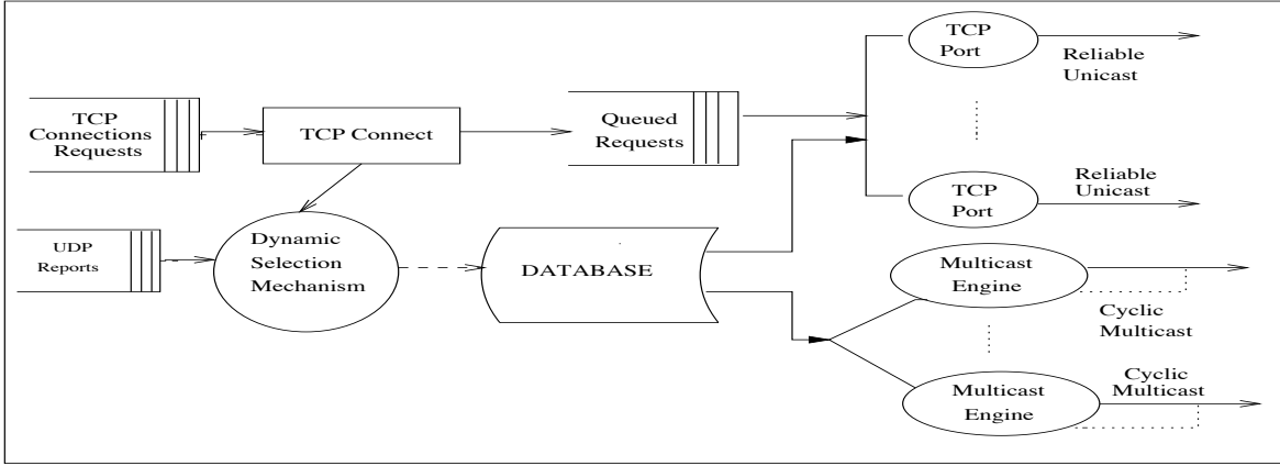
Figure 1. The Site Distribution Selection Mechanism
