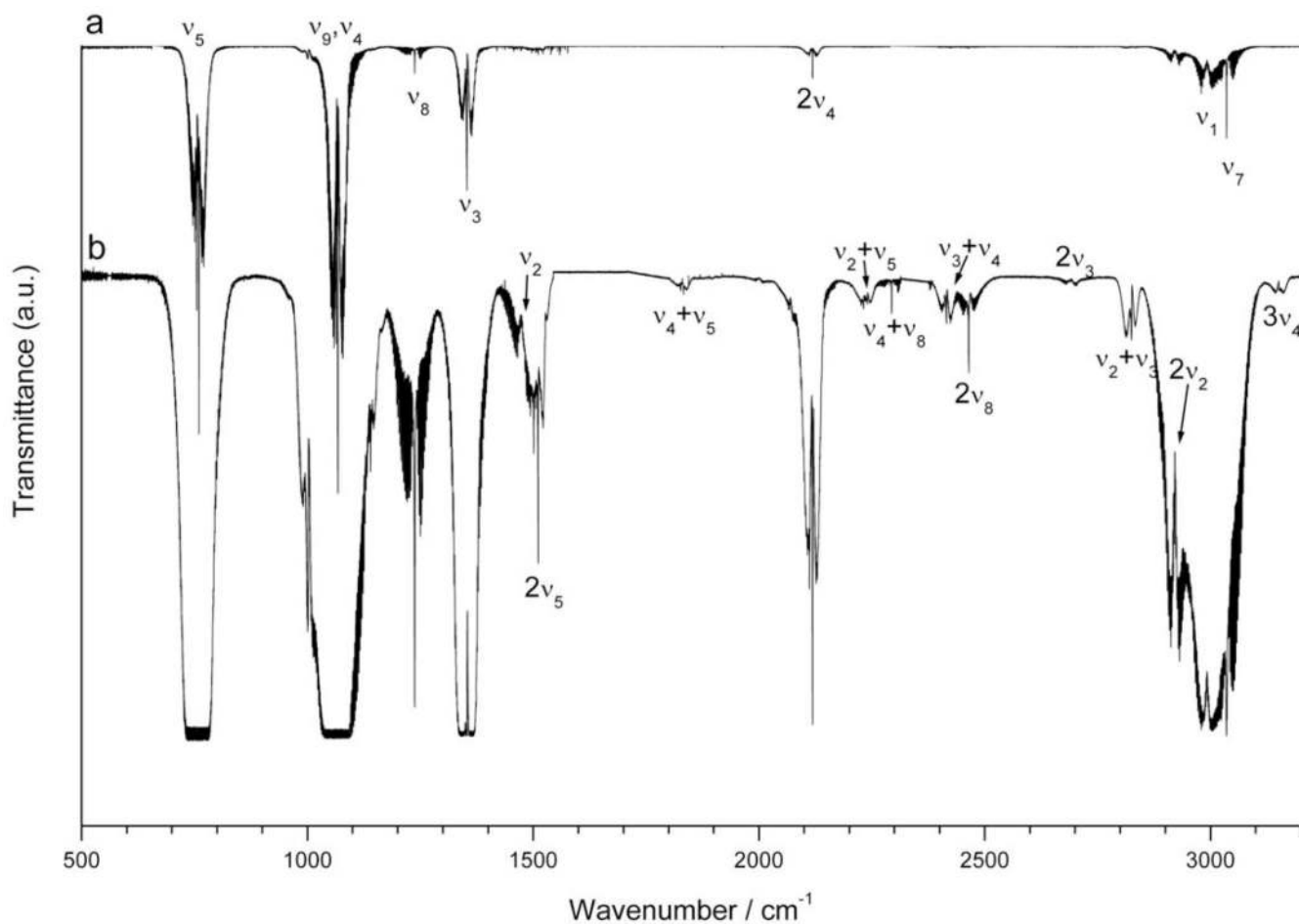
Figure 3. Survey spectra ( 500 - 3200 \text{ cm}^{-1} ) of \text{CH}_2\text{ClF} (resolution = 0.2 \text{ cm}^{-1} , path length = 134 \text{ mm} , room temperature). Traces (a) and (b) refer to the spectrum recorded with a sample pressure of 41.2 \text{ Pa} and 23 \text{ kPa} , respectively. Trace (b) displaced for clarity. Some relevant bands are labeled.
