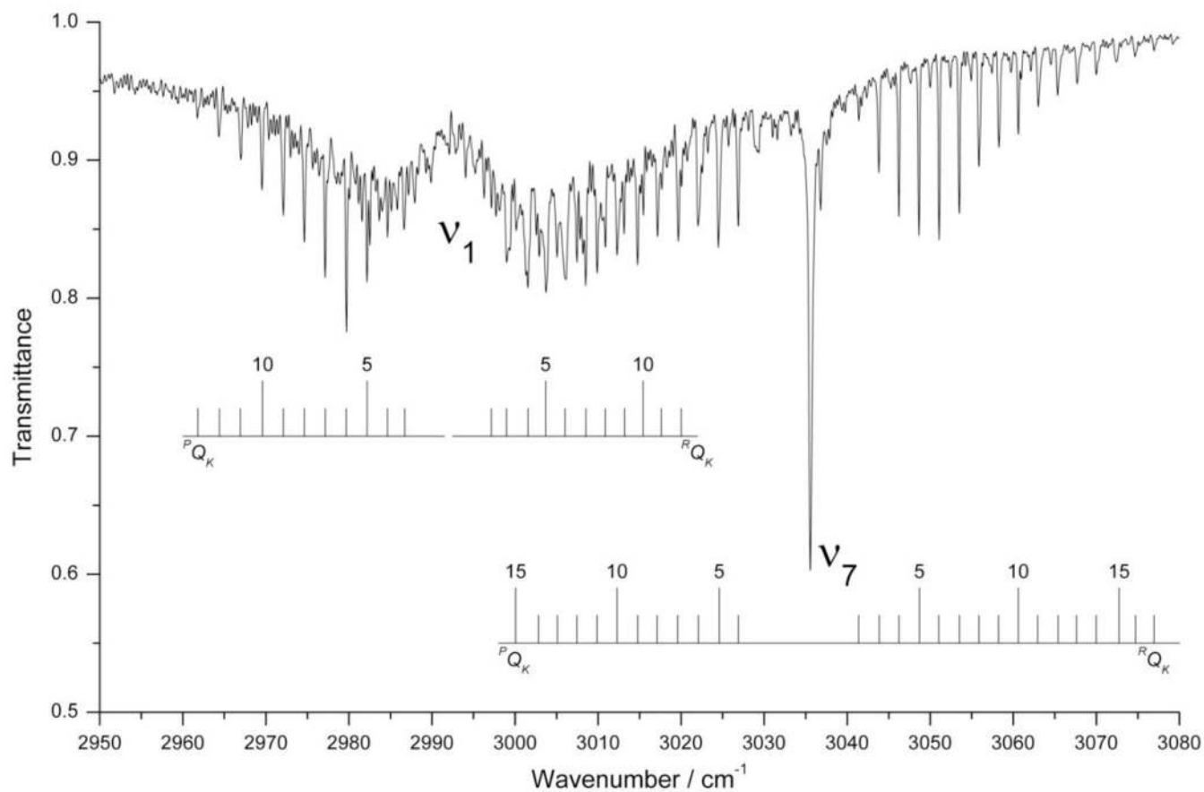
Figure 5. Details of the partially resolved rotational structures of the \nu_1 (A') and \nu_7 (A'') fundamentals in the 2950 – 3080 cm -1 spectral region (resolution = 0.2 cm -1 , sample pressure = 926 Pa, path length = 134 mm, room temperature).
