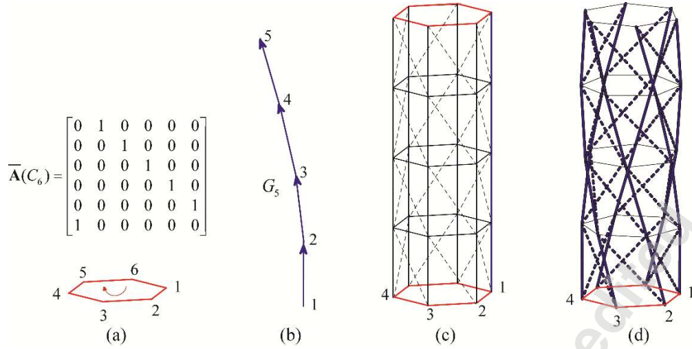
Figure 8 Cylinders expressed by directed graph products of weighted graphs in 3D space: (a) a directed cycle
