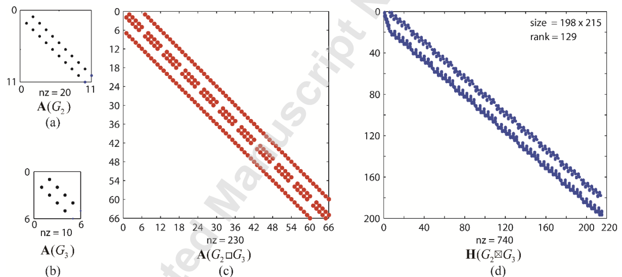
Figure 6 Distribution patterns of nonzero entries of involved matrices for the four-fold origami shown in Fig.
