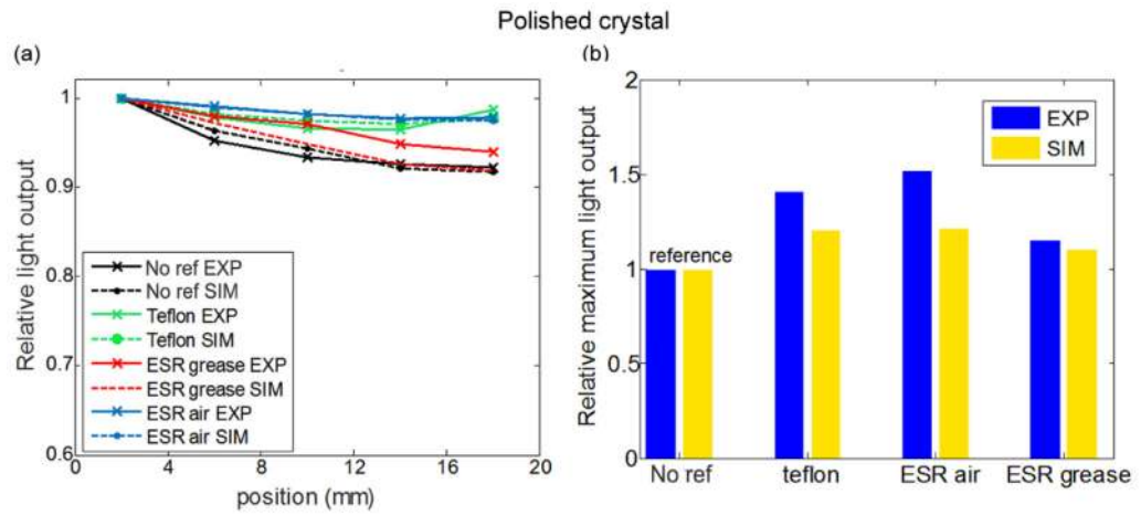
Figure 12. Light output for polished crystals with no reflector, Teflon, or ESR (air-coupled or grease-coupled). a) Normalized outputs for experiments (EXP) and simulations (SIM). b) Maximum light outputs, taken at the depth closest to the photodetector (2 mm).
