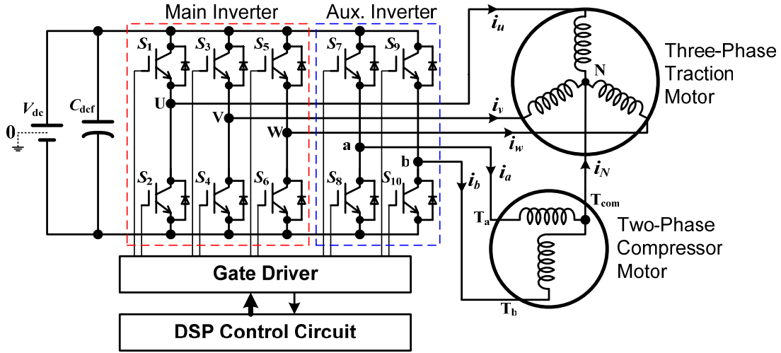
Fig. 4. Proposed integrated system for driving a three-phase traction motor and a two-phase compressor motor.
