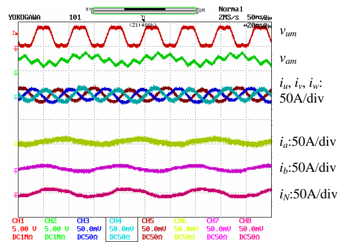
(b) With the zero-sequence voltage cancellation. Main motor at 700 rpm, two-phase motor at 500 rpm. Time: 20ms/div.
