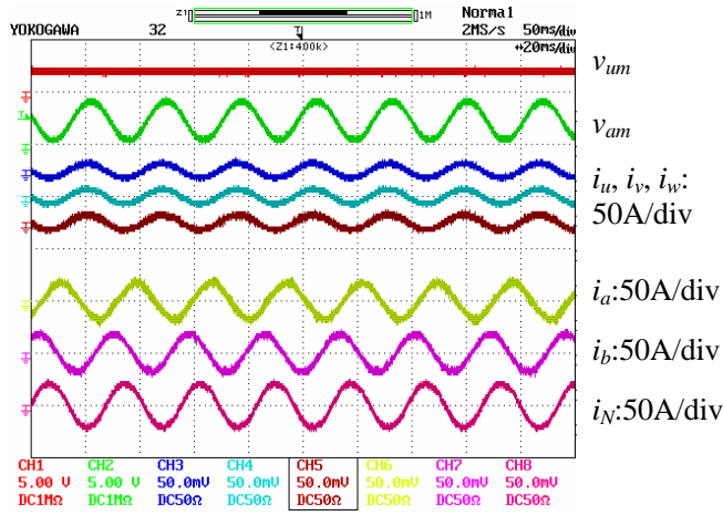
(a) Main motor is not running while two-phase motor is loaded with 14.6 N·m at 1000 rpm. Time: 20ms/div.
