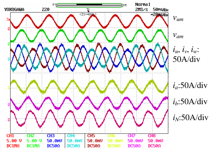
(g) Main motor loaded with 90 N-m at 685 rpm, two-phase motor loaded with 14.8 N-m at 1100 rpm. Time: 20ms/div.
