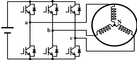
(a) A typical adjustable speed drive employing a three-phase inverter and motor.
