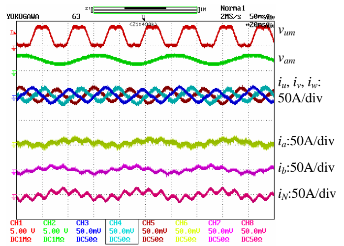
(a) Without the zero-sequence voltage cancellation. Main motor at 700 rpm, two-phase motor at 500 rpm, no load. Time: 20ms/div.
