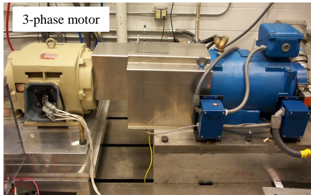
(a) Main motor mounted on a 100 HP dynamometer test bed
