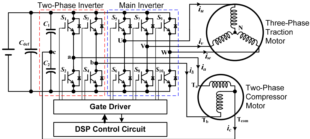
Fig. 3. A straightforward way for integrating the two-phase compressor drive into a three-phase traction motor drive system.
