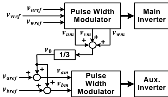
Fig. 6. PWM scheme for zero-sequence component cancellation.
