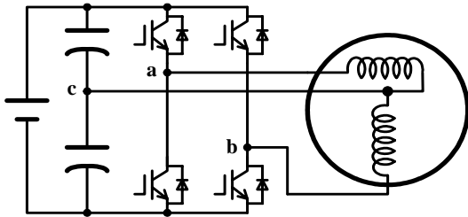
(b) A low-cost two-phase motor drive using four switches and two capacitors
