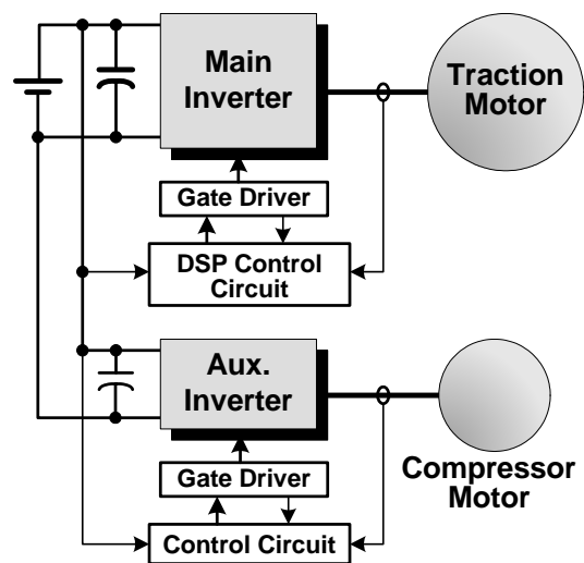
Fig. 1. A conventional traction and compressor motor drive configuration using two separate inverters.
