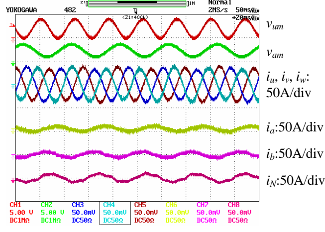
(c) Main motor is loaded with 90 N·m at 685 rpm with unloaded two-phase motor at 750 rpm. Time: 20ms/div.
