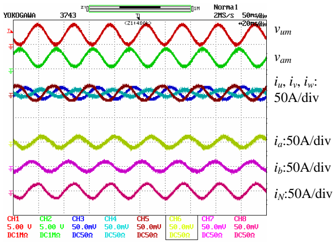
(d) Main motor at 700 rpm, no load, Two-phase motor loaded with 9.5 N-m at 1000 rpm. Time: 20ms/div.
