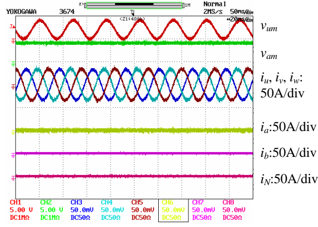
(b) Main motor is loaded with 90 N·m at 685 rpm, while two-phase motor is not running. Time: 20ms/div.
