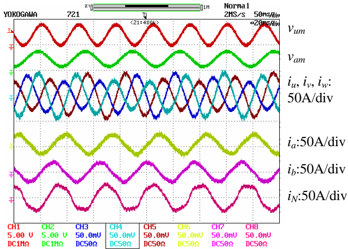
(f) Main motor loaded with 90 N-m at 685 rpm, two-phase motor loaded with 14.9 N-m at 750 rpm. Time: 20ms/div.
