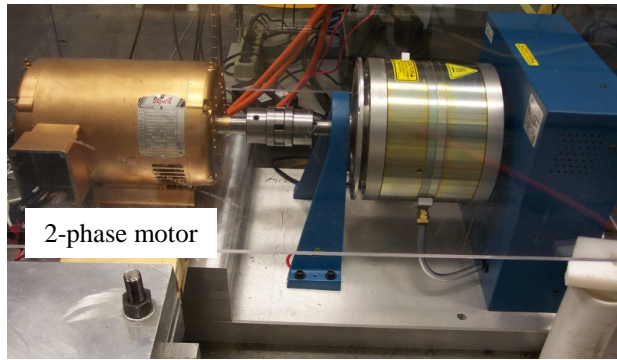
(b) Two-phase motor connected to a hysteresis dynamometer
