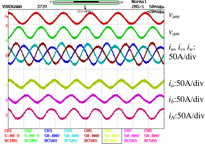
(e) Main motor loaded with 85 N-m at 550 rpm, two-phase motor loaded with 11 N-m at 1000 rpm. Time: 20ms/div.
