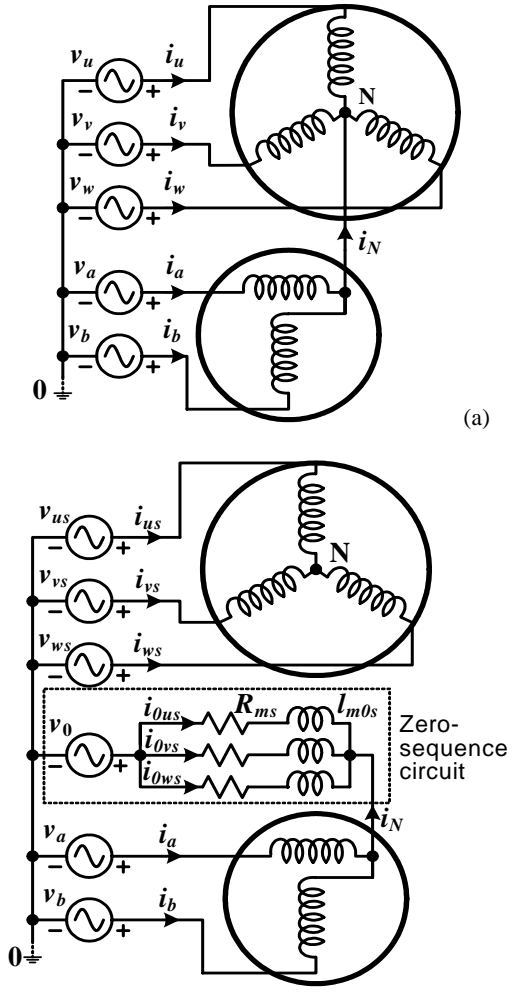
Fig. 5. Equivalent circuits; (a) showing inverter phase legs as voltage sources, and (b) showing the zero-sequence circuit of the main motor as the current return path of the two-phase motor.
