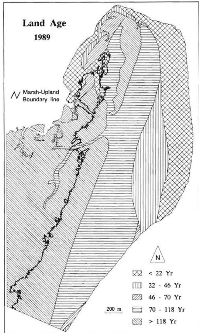
Figure 3. The spatial pattern of land age structure on northern Hog Island.
