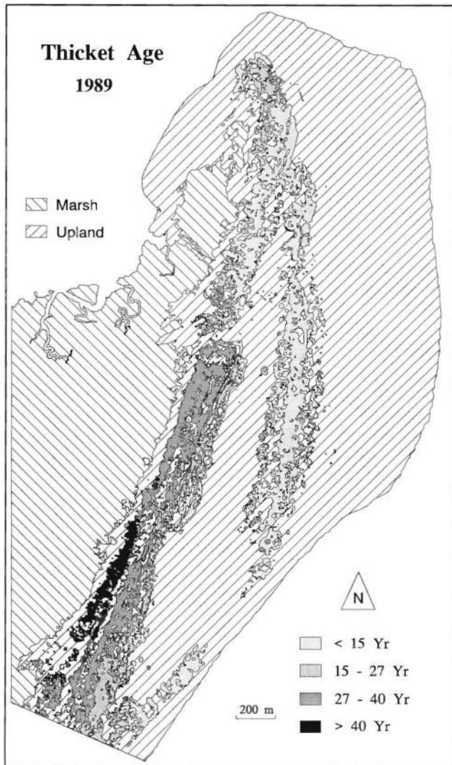
Figure 2. The spatial pattern of shrub thicket age structure on northern Hog Island.
