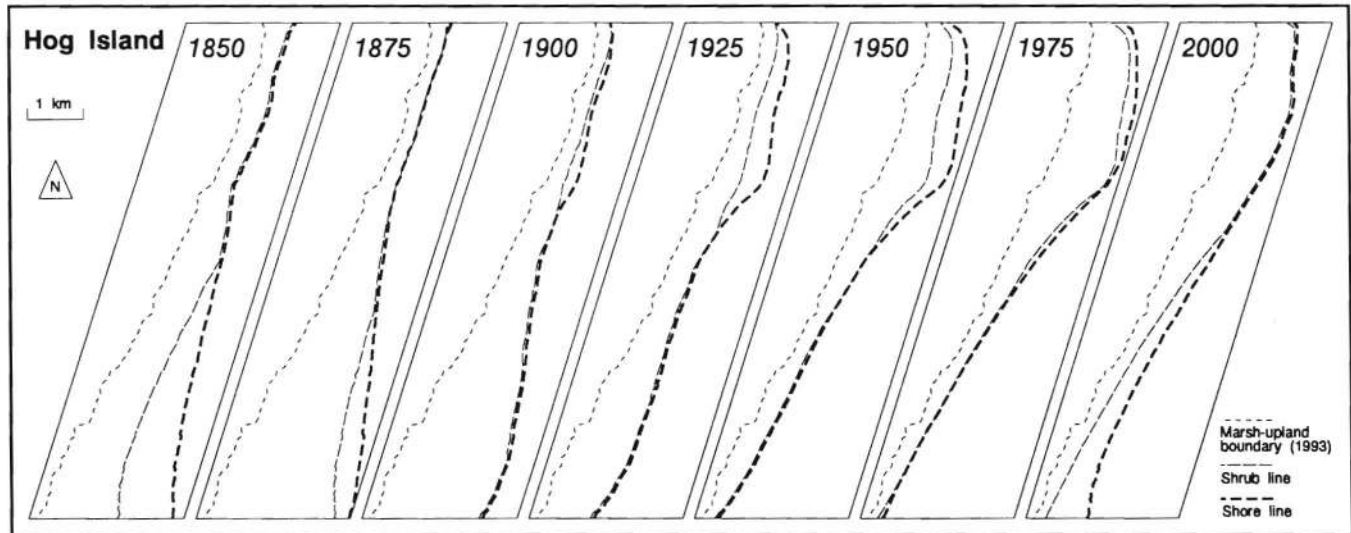
Figure 7. The temporal changes and interactions of shoreline and shrub line positions on Hog Island.
