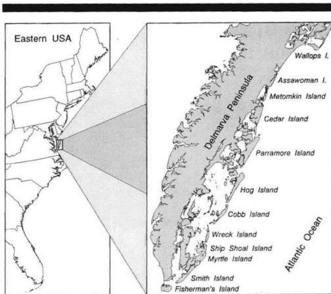
Figure 1. The study site location.
