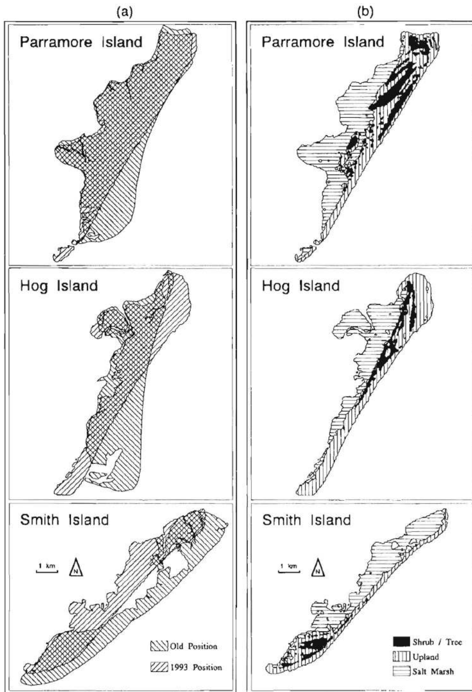
Figure 8. The comparisons of 1993 shoreline positions with 1852 (Smith) or 1871 (Parramore and Hog) shoreline positions (a) and the distributions of shrub thickets/forests on the three barrier islands of Virginia (b)
