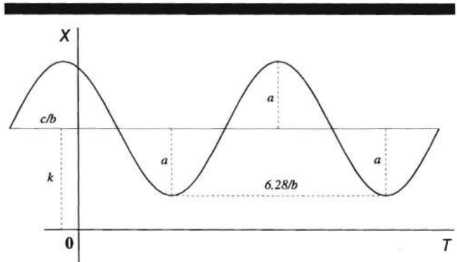
Figure 5. The four parameters of the sine function used for modeling cyclic shoreline changes.
