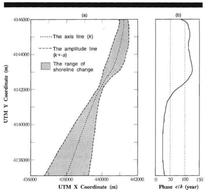
Figure 6. Parameters values of a sine model for Hog Island.
