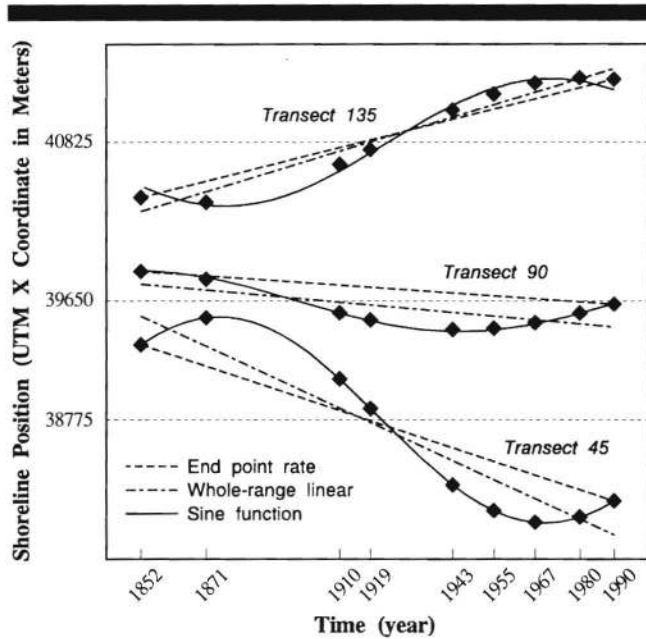
Figure 4. Comparisons of three different models for simulation shoreline changes with time on Hog Island.
