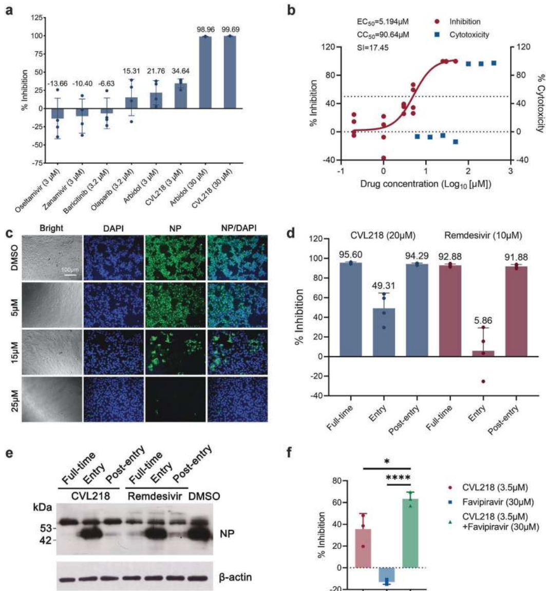
Fig. 2 The in vitro anti-SARS-CoV-2 activities of the tested drugs in Vero E6 cells. a The preliminary in vitro antiviral activities of oseltamivir at 3 \mu M, zanamivir at 3 \mu M, baricitinib at 3.2 \mu M, olaparib at 3.2 \mu M, arbidol at 3 \mu M and 30 \mu M, and CVL218 at 3 \mu M and 30 \mu M, respectively, were detected in Vero E6 cells infected with SARS-CoV-2 at an MOI of 0.05. The viral yield in the cell supernatant was then quantified by qRT-PCR. Results are shown as mean \pm SD over four replicates. b The concentration-dependent inhibition curve of CVL218 against SARS-CoV-2 replication and its cytotoxicity results. Viral infection and drug treatment at different concentrations were performed as mentioned above. Cytotoxicity of CVL218 to Vero E6 cells was measured by the CCK8 assays. c Visualization of virus nucleoprotein (NP) expression of the infected cells upon treatment of CVL218 at 48 h post the SARS-CoV-2 infection using fluorescence microscopy. d Time-of-addition results on the inhibition of CVL218 and remdesivir against SARS-CoV-2 in vitro. The viral inhibitory activities of CVL218 and remdesivir were measured at “full-time”, “entry”, and “post-entry” stages, respectively. Results are shown as mean \pm SD over four replicates. e Virus NP expression in the infected cells upon the treatment of CVL218 and remdesivir was analyzed by western blot. f In vitro inhibitory activities against SARS-CoV-2 replication of favipiravir (30 \mu M), CVL218 (3.5 \mu M) and a combination of both drugs (30 \mu M favipiravir + 3.5 \mu M CVL218). The concentrations were selected according to the EC 25 values of individual drugs against SARS-CoV-2 in vitro. Viral infection and drug treatment were performed as mentioned above. Results are shown as mean \pm SD over three replicates, and the significances were measured by p -values from t -tests. * and **** stand for p -value < 0.05 and p -value < 0.0001, respectively
