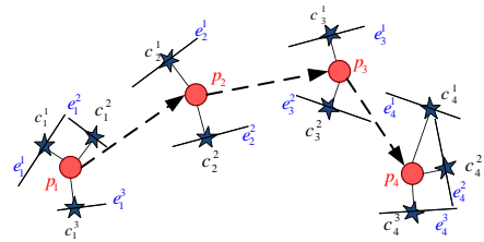
Figure 8. Candidate road segments and candidate points
