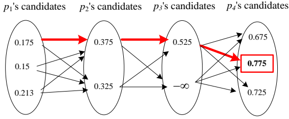
Figure 10. FindSequence process of candidate c_1^1
