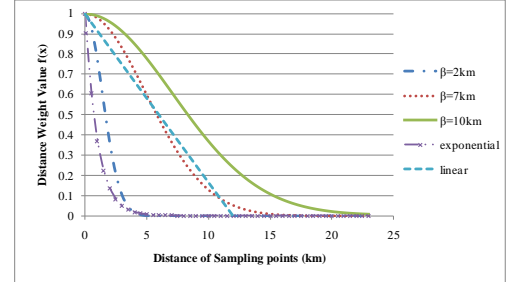
Figure 18. Different distance weight functions
