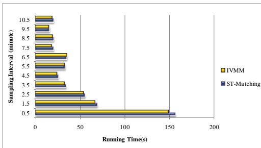
Figure 17. Running time (ST-Matching V.S. IVMM)
