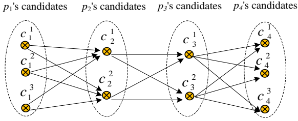
Figure 9. Candidate graph
