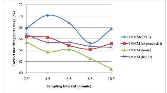
Figure 19. Impact of different distance weight functions
