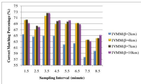
Figure 20. Impact of parameter \beta with IVMM
