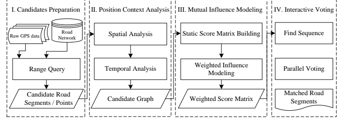
Figure 6. Overview of the IVMM algorithm
