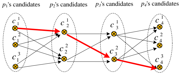
Figure 11. Matching result of IVMM algorithm
