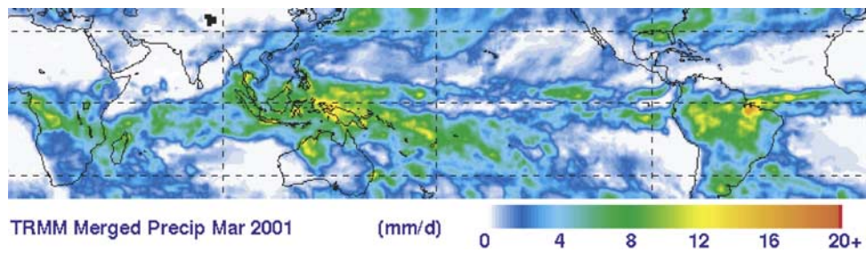
Figure 7. (a) Lightning data for March 2001 from the Lightning Imaging Sensor (LIS) (b) Precipitation data for March 2001 from the Tropical Rainfall Measuring Mission (TRMM).
