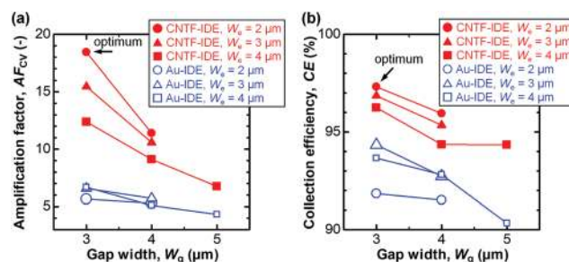
Fig. 4 (a) The amplification factor ( AF_{CV} ) and (b) the collection efficiency (CE) with CV with different electrode structures. The data with the optimum electrode structure ( W_e = 2 \mu m and W_g = 3 \mu m ) are shown with arrows.
