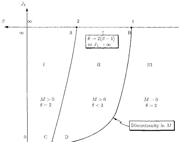
Fig. 1. Schematic phase diagram in the \beta (inverse temp.)- J_1 (nearest neighbor coupling) plane. M denotes the magnetization (or percolation density) and \theta the power law decay exponent for the truncated two-point function. It is conjectured that \theta = 2(M^2\beta - 1) in region II and \theta = 0 on the curve BD
