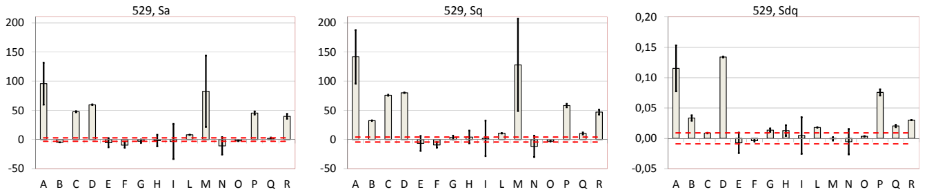
Figure 3. Left: S_a deviations for 529 type samples (periodic profile), expressed in nm. Centre: S_q deviations for 529 type samples, expressed in nm. Right: S_{dq} deviations for 529 type samples, dimensionless. Red dashed lines (---) indicate the expanded uncertainty of AFM reference measurements. Bars on histograms indicate the expanded uncertainty of the measurements stated by the participants.
