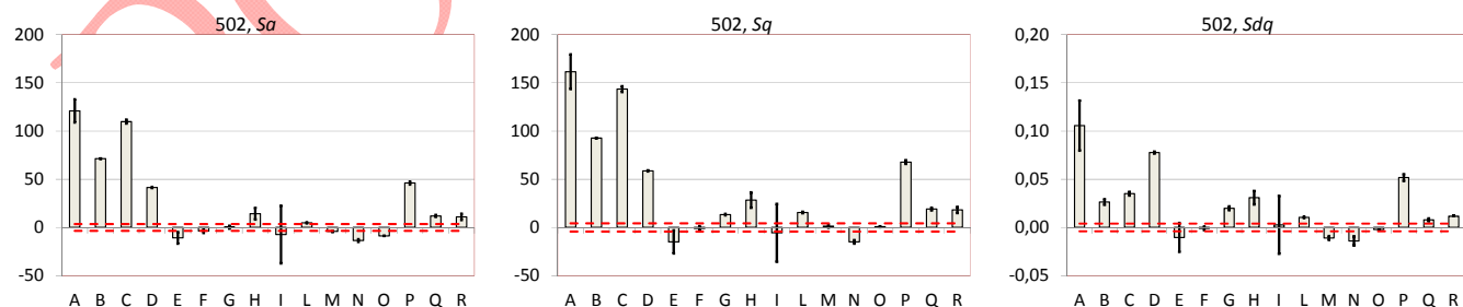
Figure 2. Left: S_a deviations for 502 type samples (random profile), expressed in nm. Centre: S_q deviations for 502 type samples, expressed in nm. Right: S_{dq} deviations for 502 type samples, dimensionless. Red dashed lines (- -) indicate the expanded uncertainty of AFM reference measurements. Bars on histograms indicate the expanded uncertainty of the measurements stated by the participants.
