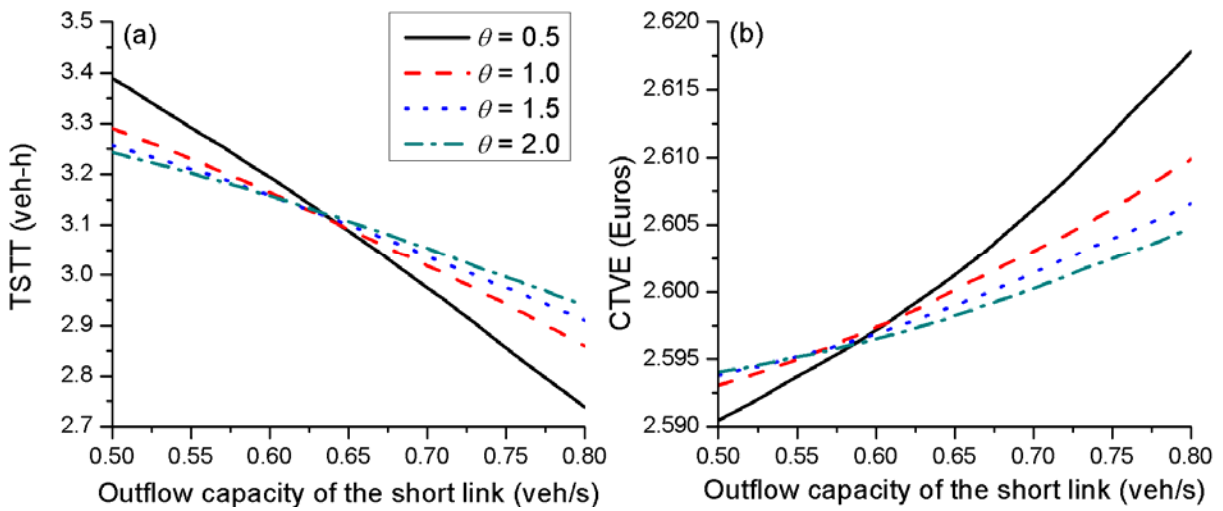
Fig. 14. The influence of outflow capacity improvement of a link on network performance in Example 4.
